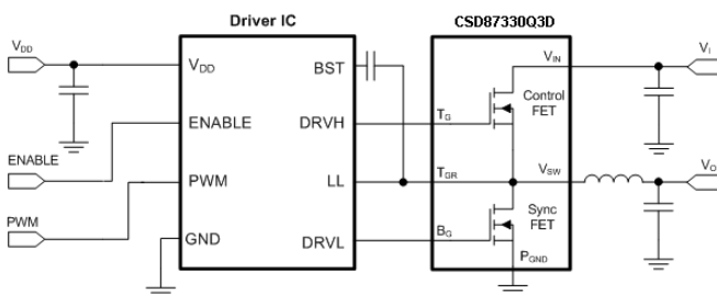
TYPICAL CIRCUIT
