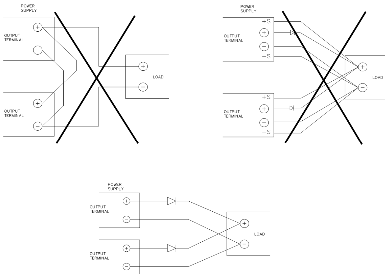
Fig. 11-3 Parallel for Redundant Operation
