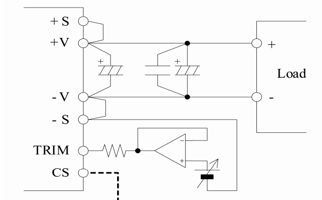
Fig. 11-1 Output Voltage Adjustment by applying external voltage (For parallel operation)
