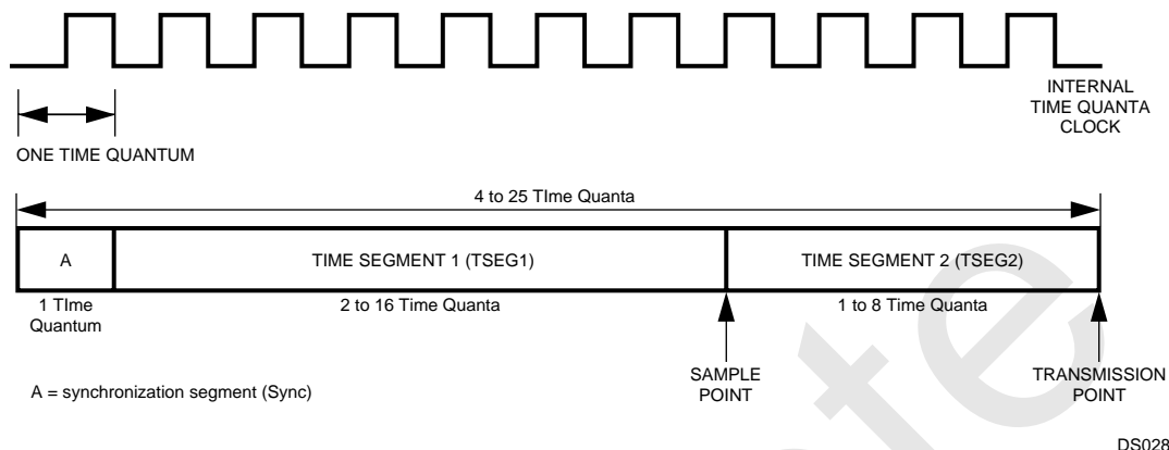
Figure 42. Bit Timing
