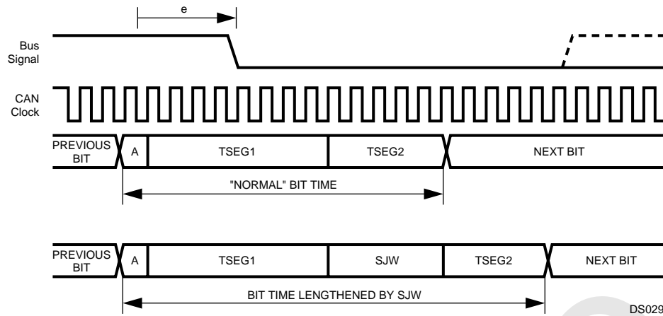
Figure 43. Resynchronization ( e > SJW )
