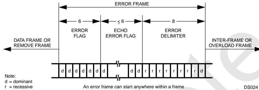
Figure 38. Error Frame
