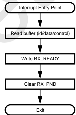
Figure 53. Buffer Read Routine (BUFFLOCK Enabled)
