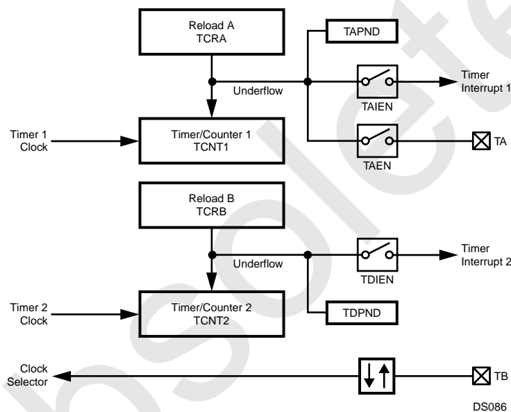
Figure 100. Dual-Independent Timer/Counter Mode
