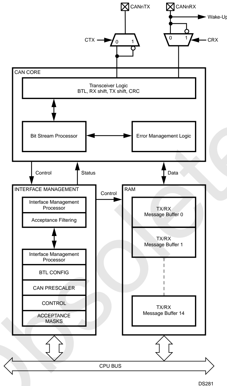
Figure 32. CAN Block Diagram
