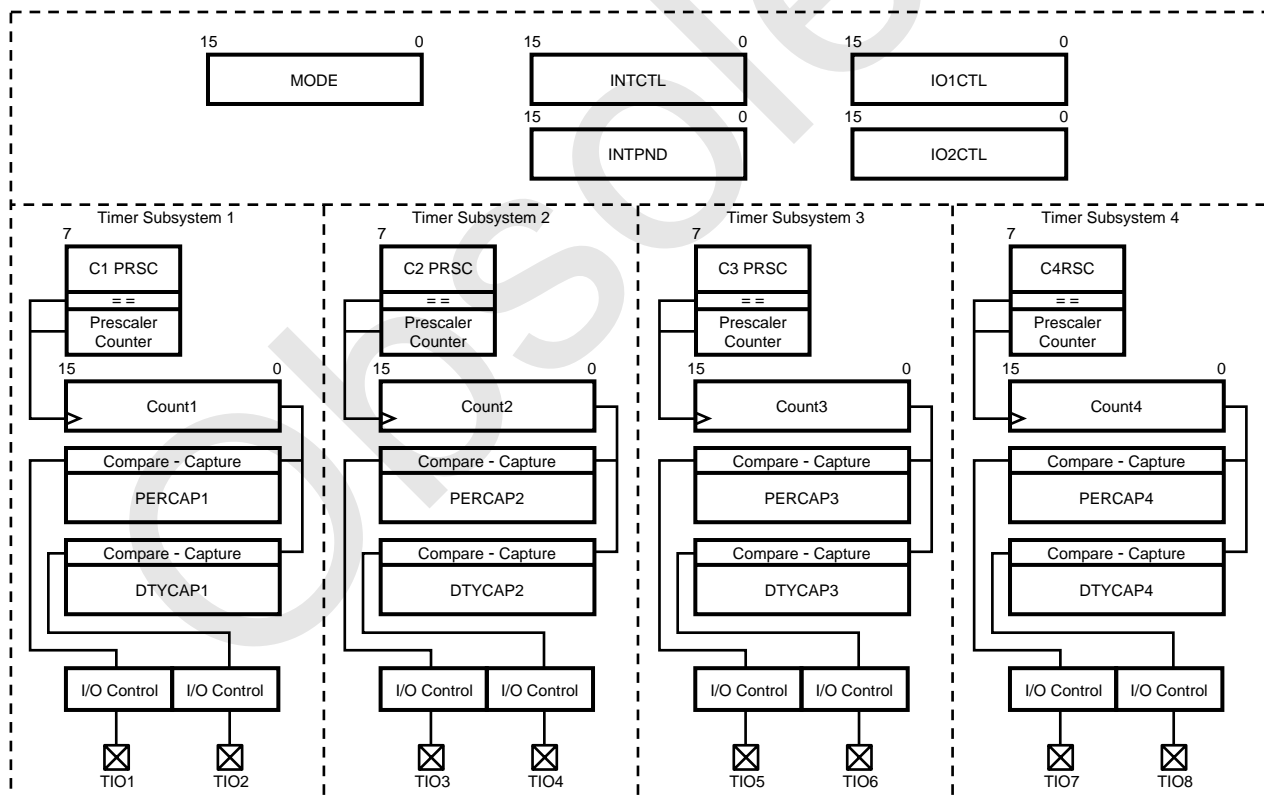
Figure 102. Versatile Timer Unit Block Diagram
