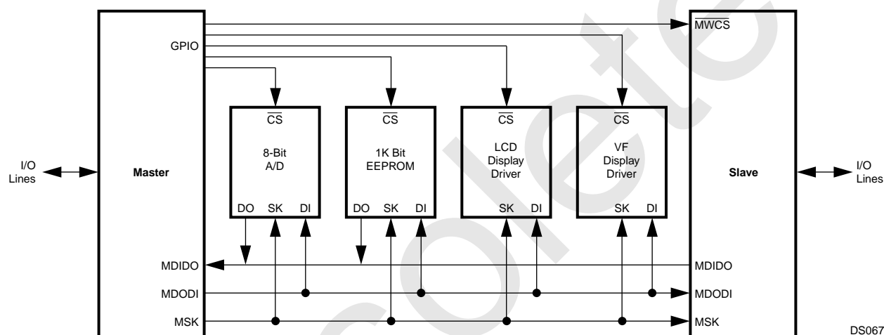
Figure 81. Microwire Interface
