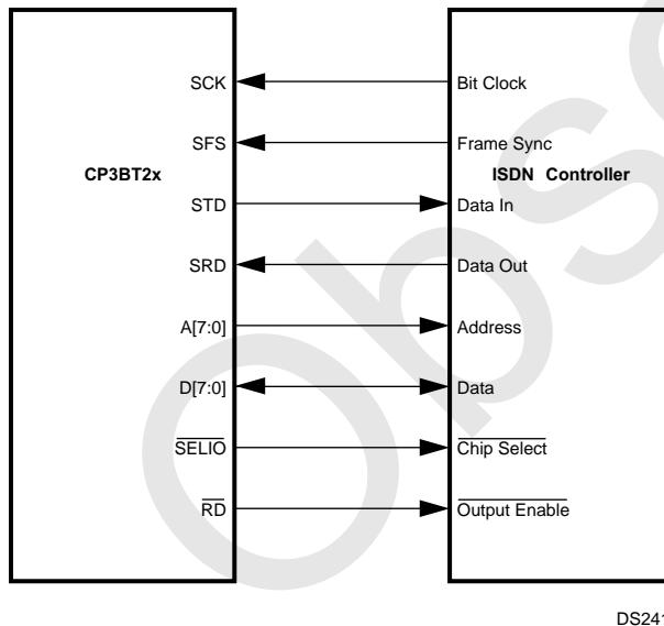
Figure 72. CP3BT23/ISDN Controller Connections
