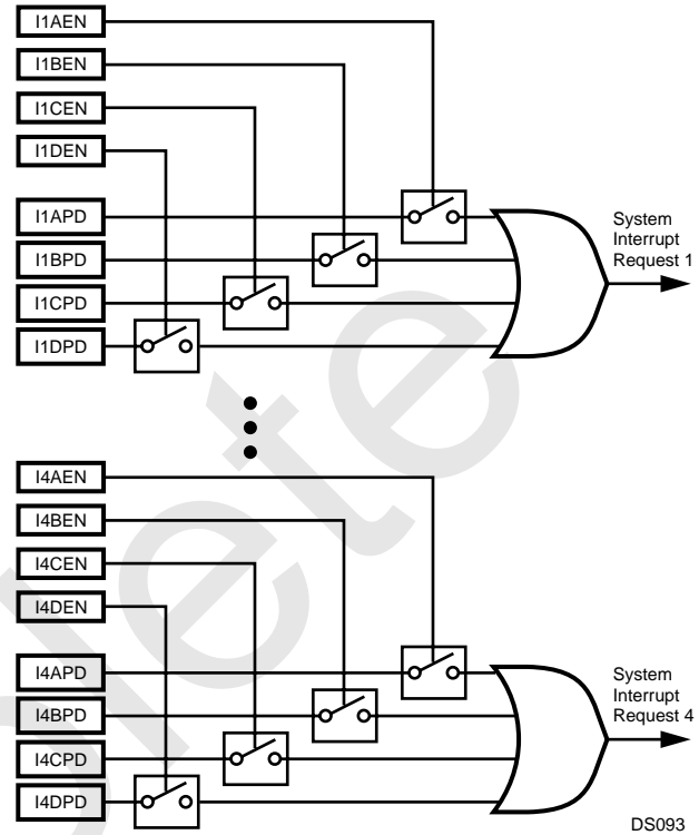
Figure 107. VTU Interrupt Request Structure
