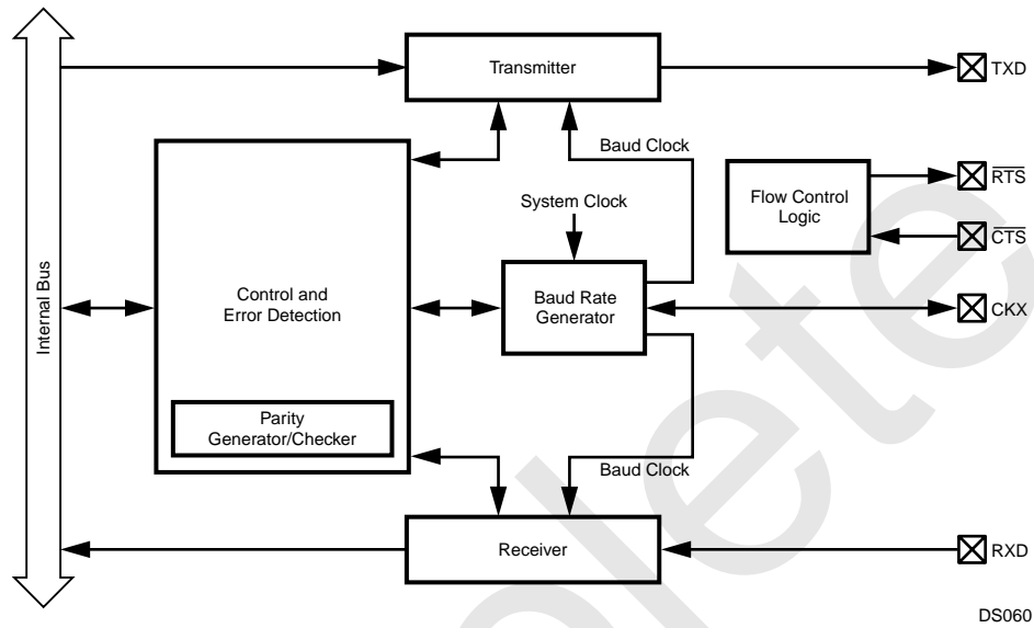
Figure 74. UART Block Diagram
