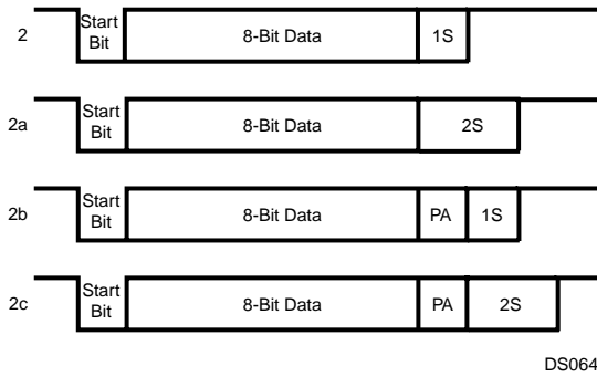
Figure 78. 8-Bit Data Frame Options
