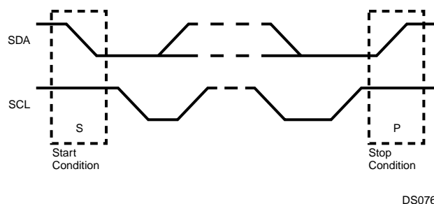
Figure 90. Start and Stop Conditions
