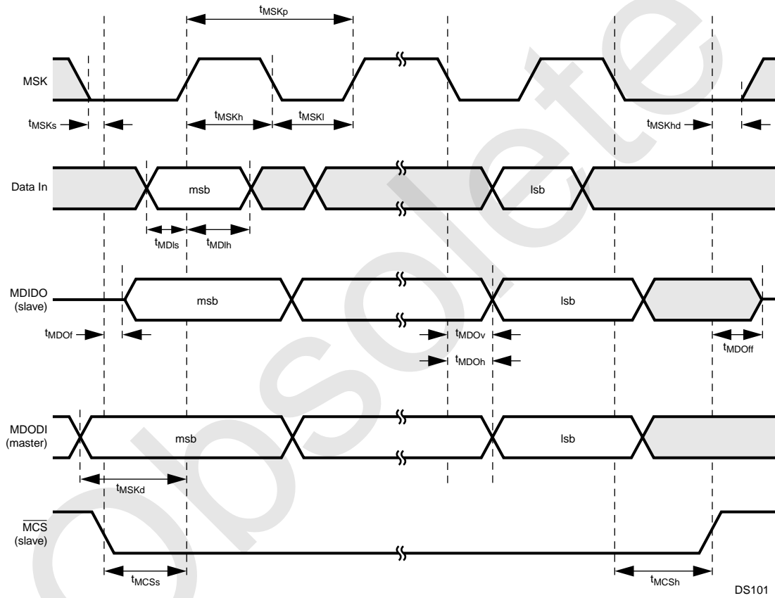
Figure 118. Microwire Transaction Timing, Normal Mode, SCIDL = 0
