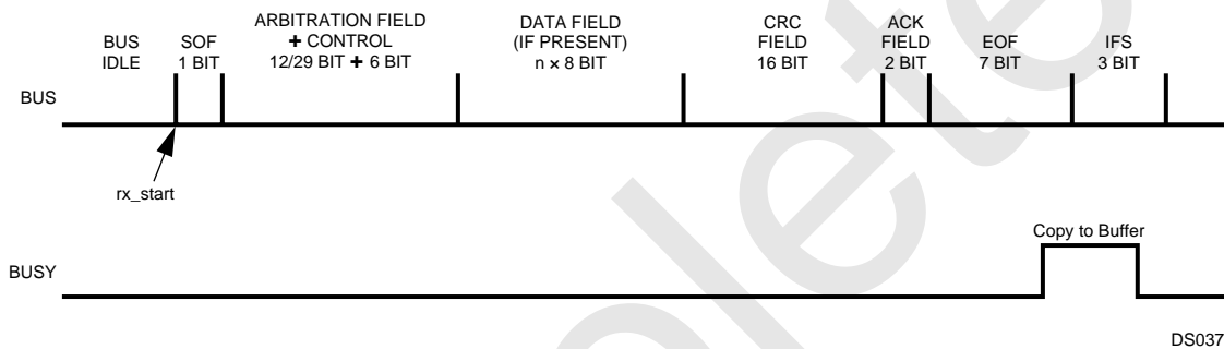
Figure 51. Receive Timing
