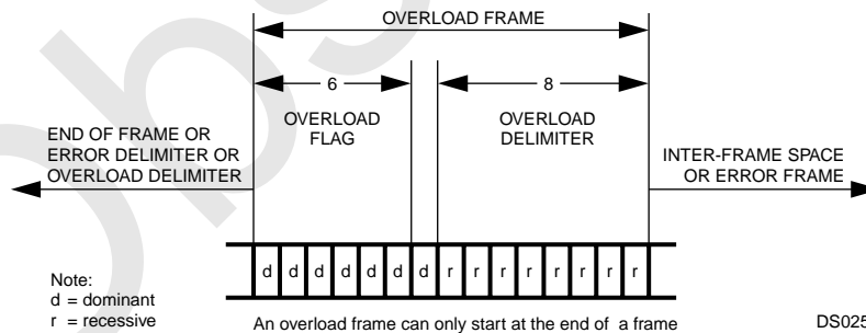
Figure 39. Overload Frame
