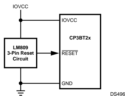
Figure 8. Simple External Reset
