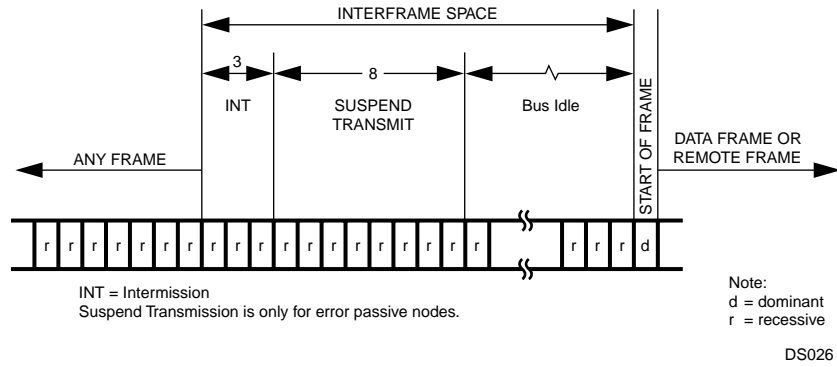
Figure 40. Interframe Space
