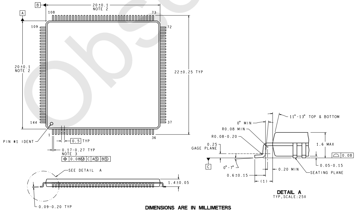
Figure 137. LQFP-144 Package
