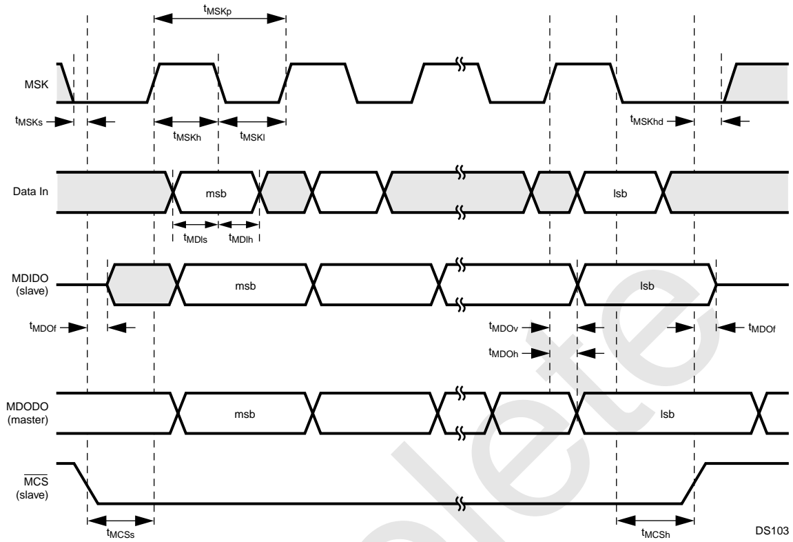
Figure 120. Microwire Transaction Timing, Alternate Mode, SCIDL = 0
