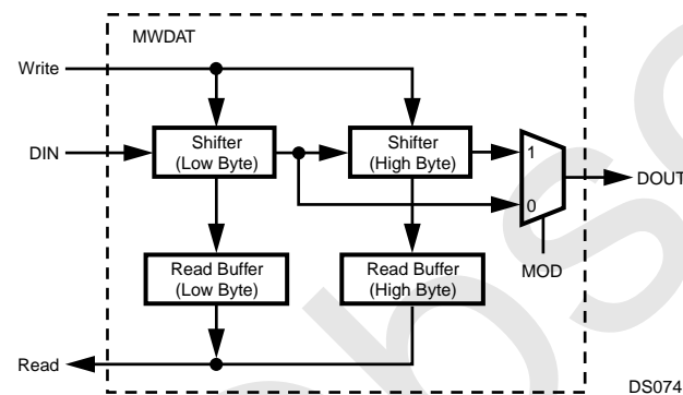
Figure 88. MWDAT Register
