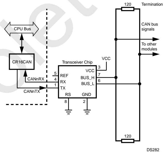
Figure 62. External Transceiver
