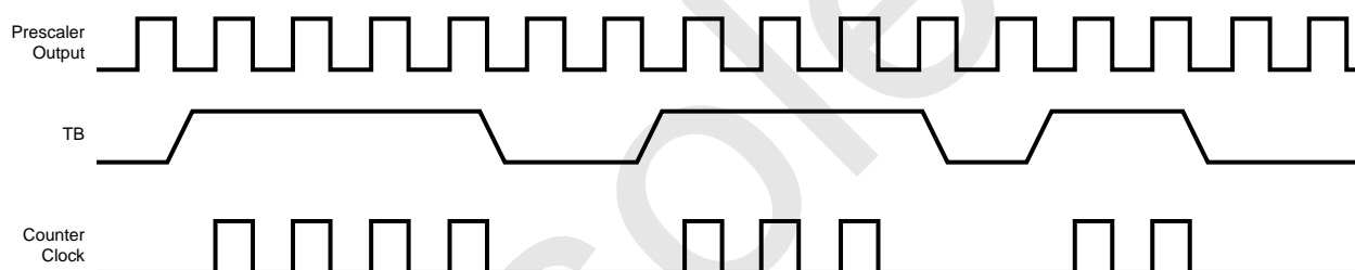
Figure 97. Pulse-Accumulate Mode
