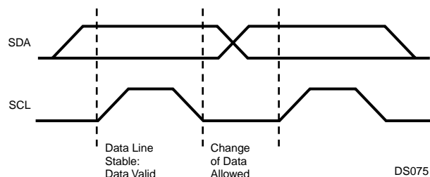
Figure 89. Bit Transfer
