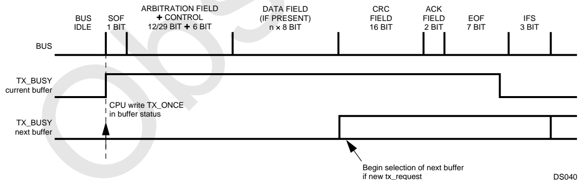
Figure 54. Data Transmission
