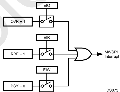
Figure 87. MWSPi Interrupts
