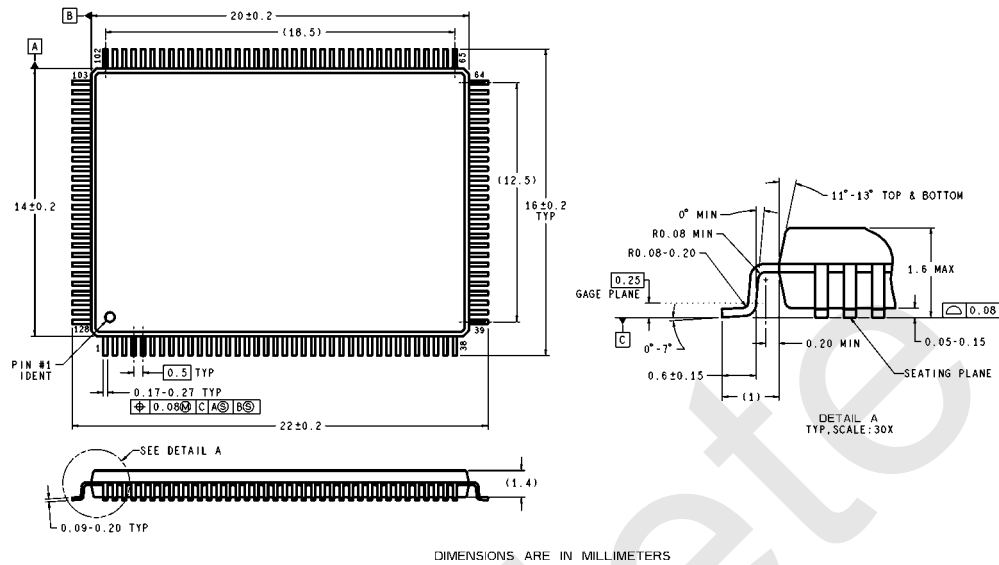
Figure 136. LQFP-128 Package
