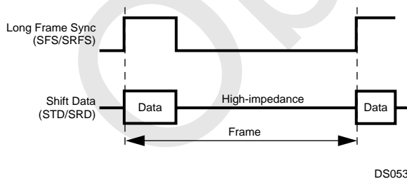
Figure 63. Normal Mode Frame
