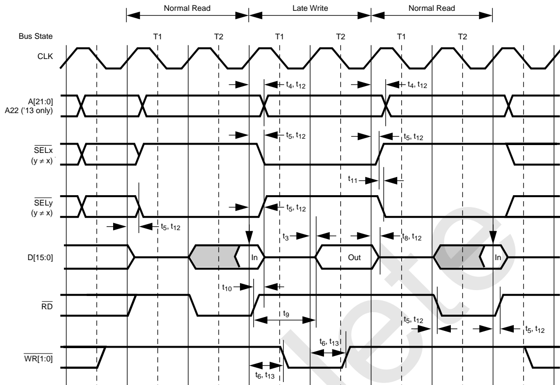
Figure 130. Late Write Between Normal Read Cycles (No Wait States)
