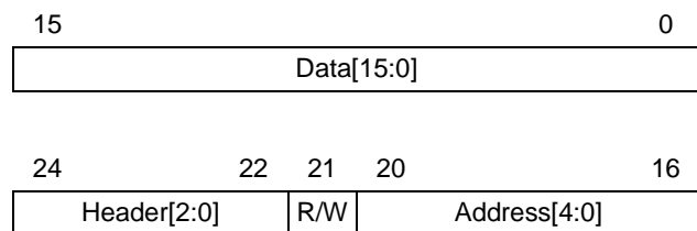
Figure 16. Serial Interface Protocol Format
