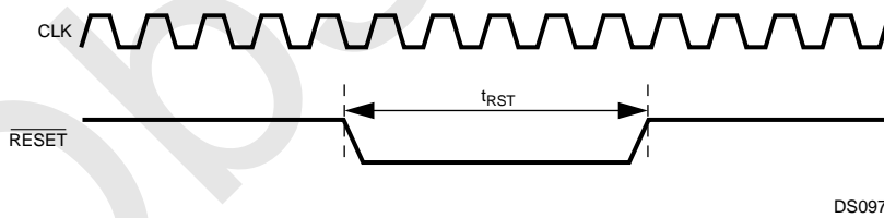
Figure 110. Non-Power-On Reset
