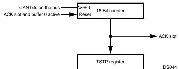
Figure 58. Time Stamp Counter
