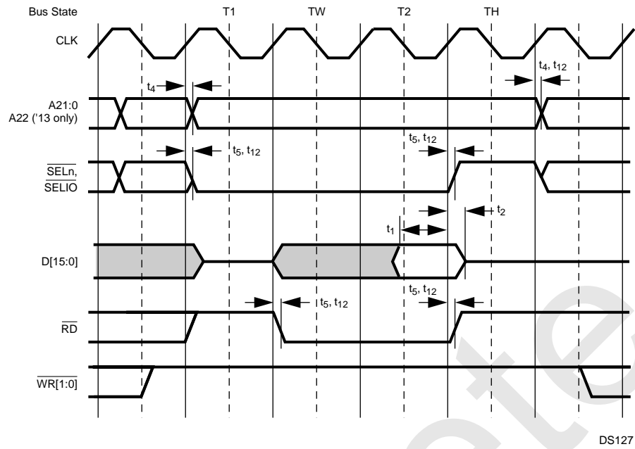
Figure 132. Normal Read Cycle (Wait Cycle Followed by Hold Cycle)
