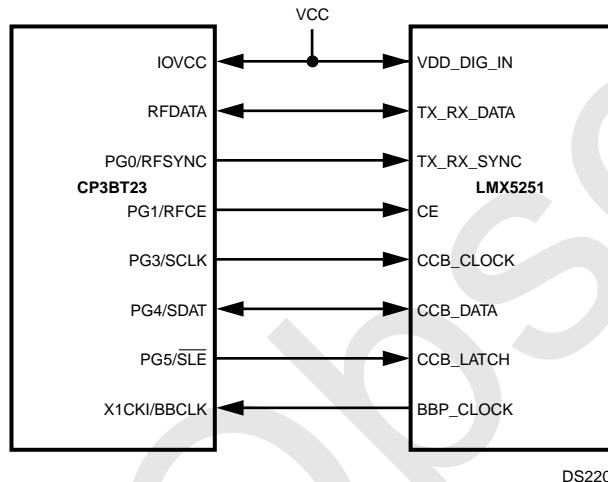
Figure 14. LMX5251 Interface
