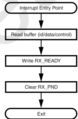
Figure 46. Buffer Read Routine (BUFFLOCK Enabled)
