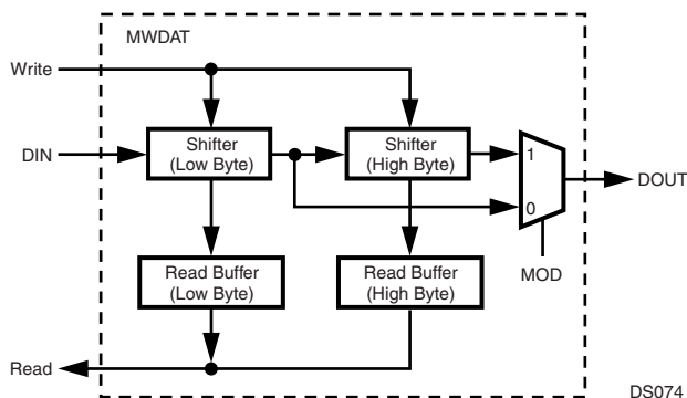
Figure 81. MWDAT Register
