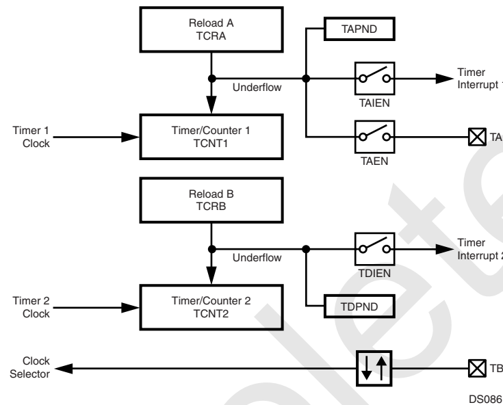
Figure 93. Dual-Independent Timer/Counter Mode
