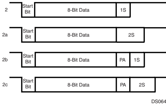
Figure 71. 8-Bit Data Frame Options
