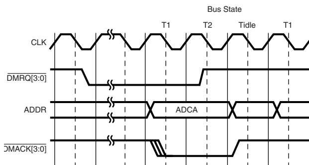
Figure 2. Direct DMA Cycle Followed by a CPU Cycle
