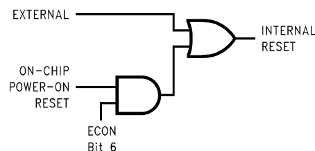
Figure 17. Reset Logic
