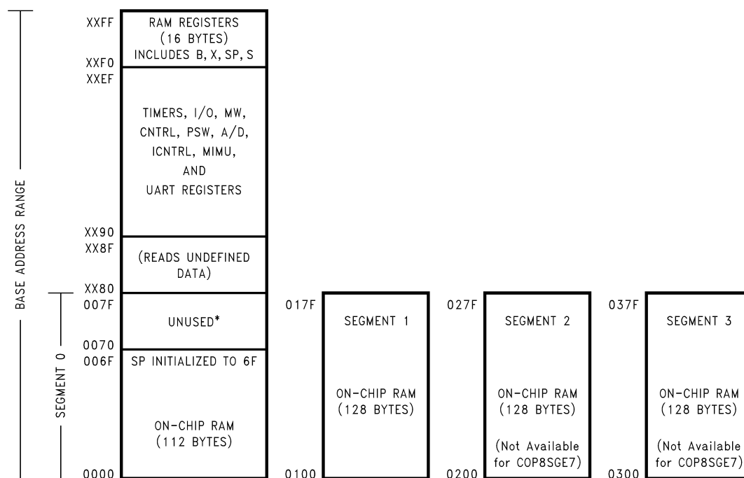
Figure 16. RAM Organization
