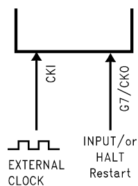
Figure 22. External Oscillator
