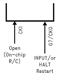
Figure 23. R/C Oscillator
