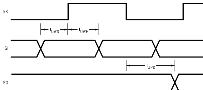
Figure 3-1. MICROWIRE/PLUS Timing
