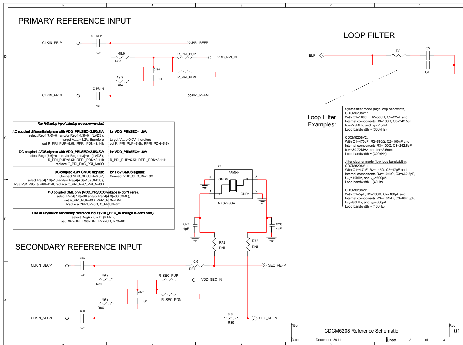
Figure 55. Schematic page 2
