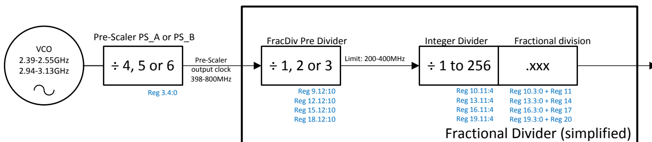
Figure 35. Fractional Output Divider Principle Architecture (Simplified Graphic, not Showing Output Divider Bypass Options)
