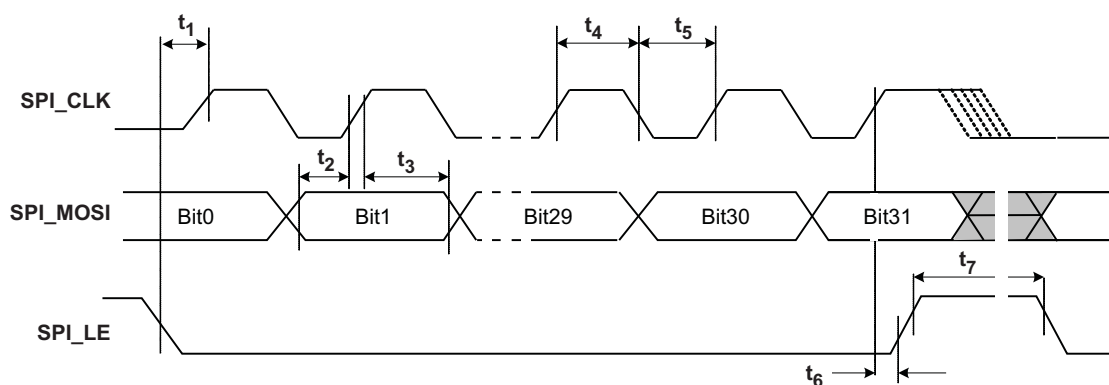
Figure 21. Timing Diagram for SPI Write Command
