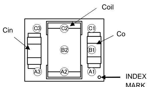
Figure 2. Pin Configuration(s)
