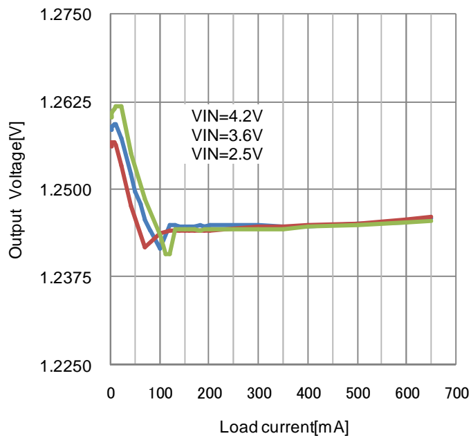
Figure 35. Load regulation PWM/PFM Auto mode
