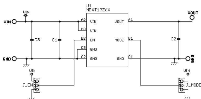
Figure 40. PCB Circuit
