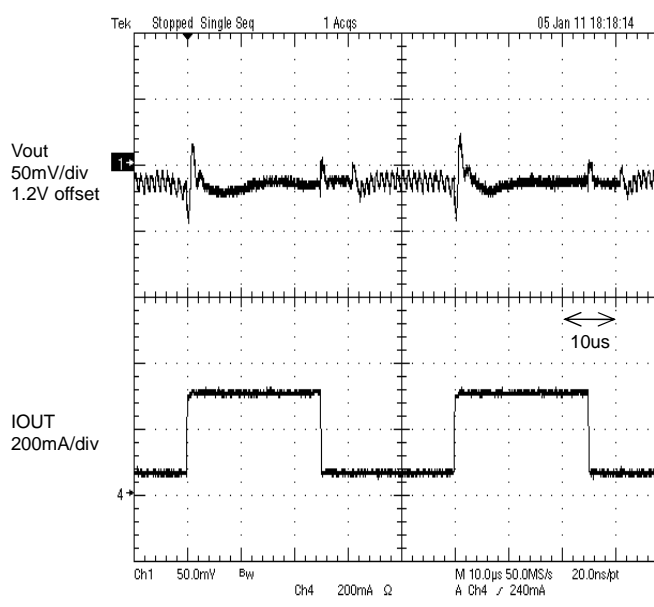
Figure 24. Load transient response 50mA to 350mA t_r=t_f=100\text{ns} , MODE : Low
