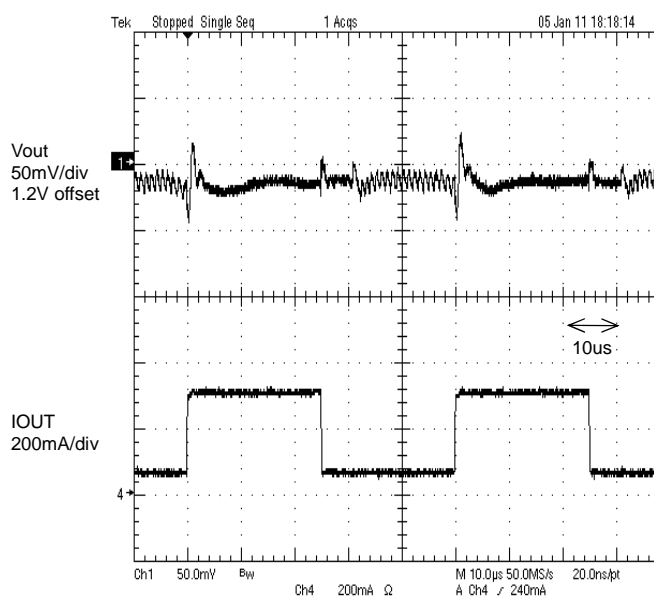
Figure 8. Load transient response 50mA to 350mA t_r=t_f=100\text{ns} , MODE : Low
