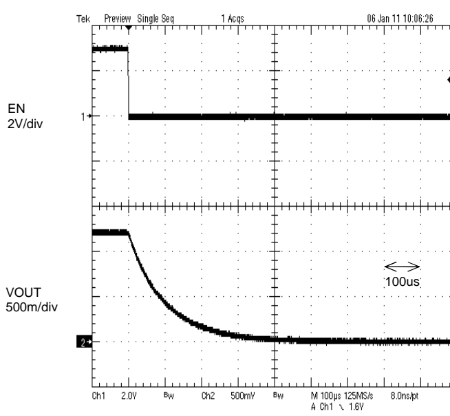
Figure 22. Shut down
