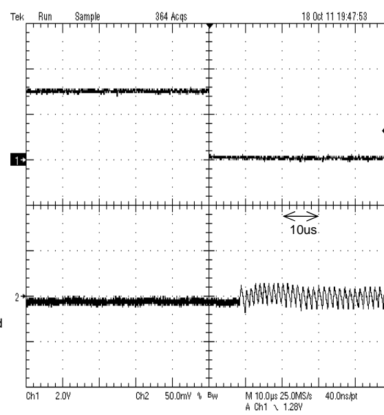
Figure 32. Mode Change Response MODE : High to Low
