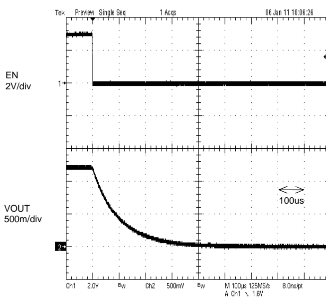
Figure 6. Shut down
