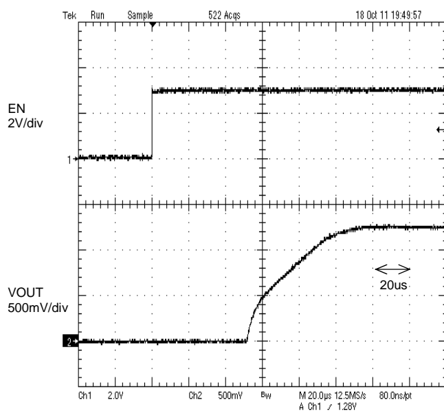
Figure 21. Start up
