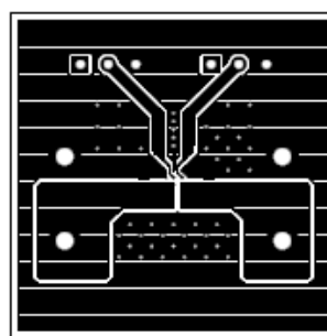
Figure 39. PCB layout (solder side)
