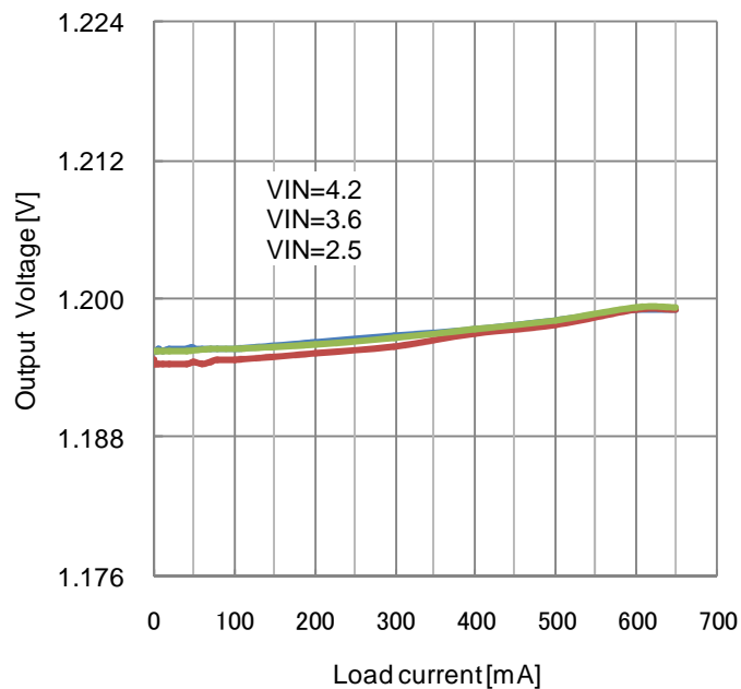
Figure 20. Load regulation PWM mode
