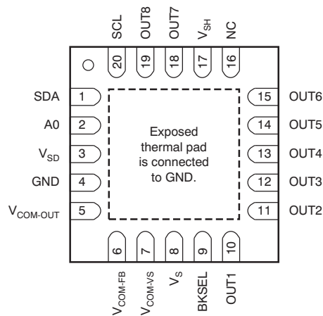
RGW PACKAGE VQFN-20 (TOP VIEW)
