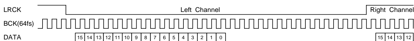
Figure 16. I 2 S Output Timing (64fs)
