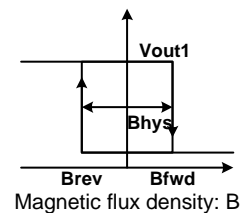
Figure 2. Output operation
