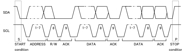
Figure 34. Data Transfer Timing
