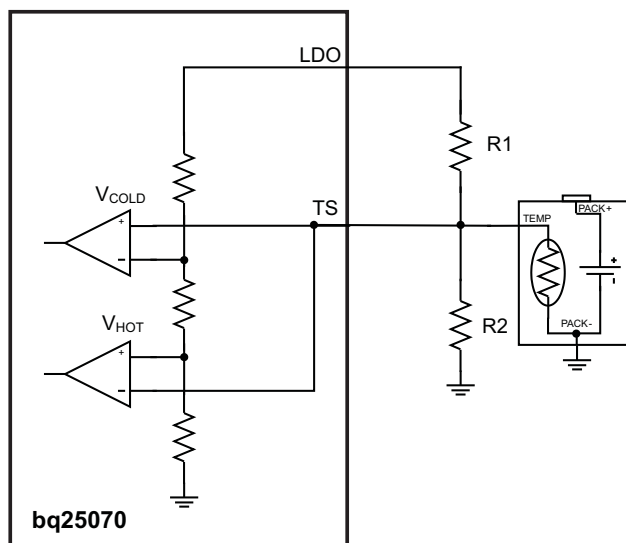
Figure 14. NTC Monitoring Function
