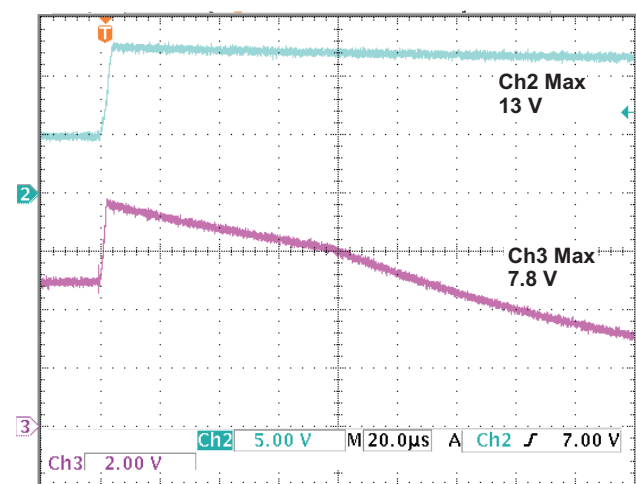
Figure 5. OVP Response for Input Step, V_{IN} = 5\text{ V to }12\text{ V} , t_r = 4\mu\text{s} . CH2 input voltage peak = 13\text{ V} , CH3 output voltage peak = 7.8\text{ V} . OVP duration is longer than Blanking time.
