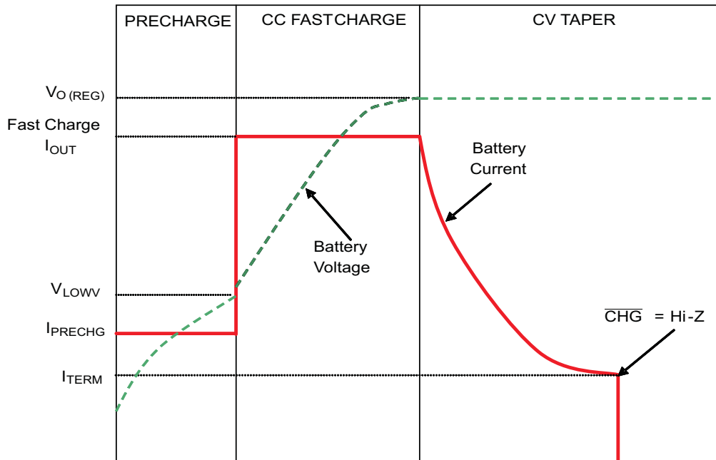
Figure 4. Charge Profile
