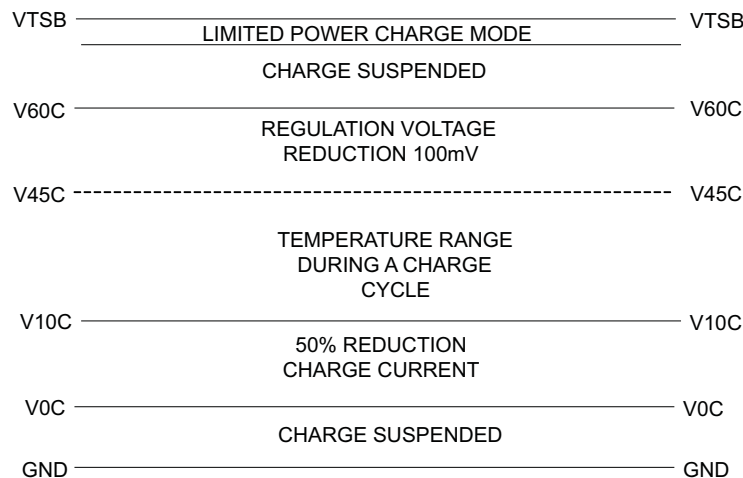
Figure 12. TS Pin, Thermistor Sense Thresholds
