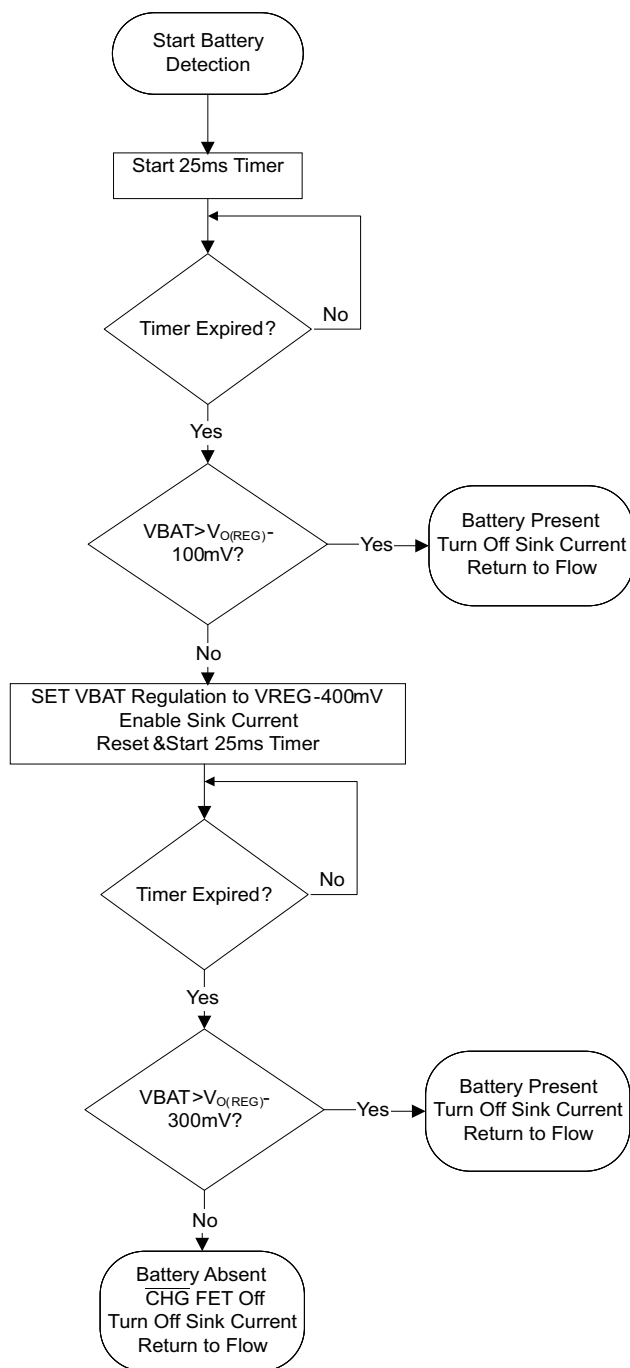
Figure 14. Battery Detection Flow Chart
