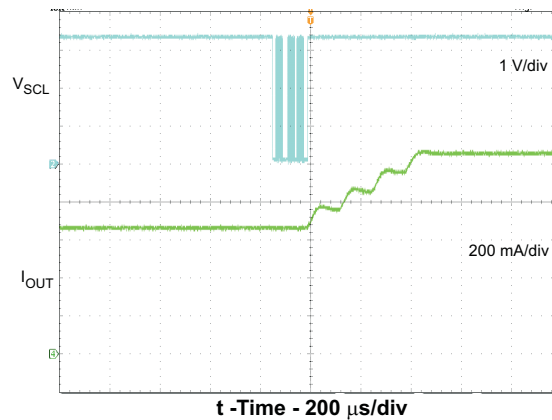
Figure 12. Charge Current Transition 550mA to 1.05A Using I²C
