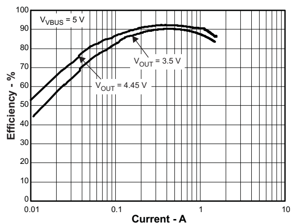
Figure 24. Charger Efficiency
