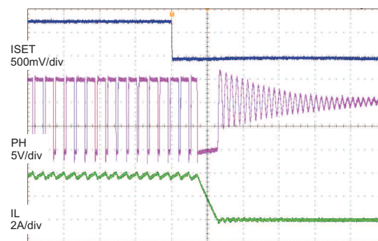
2 μs/div Figure 6. Charge Disable by ISET
