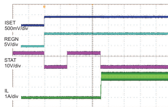
400 ms/div Figure 4. Charge Enable by ISET
