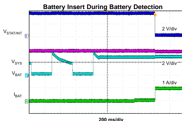
Conditions: Termination Enabled Figure 8.
