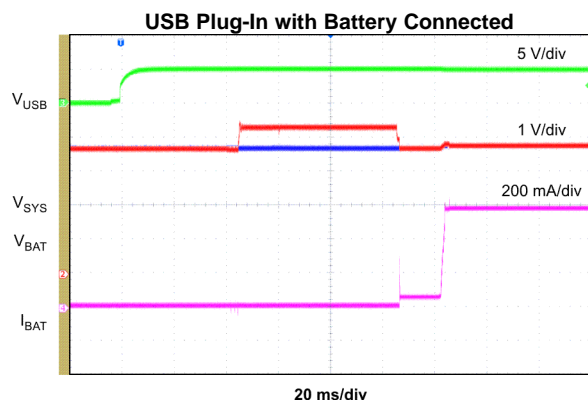
Conditions: USB500, 925mA Charge Setting Figure 5.
