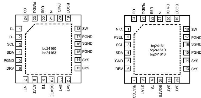
Figure 1. 24-Pin VQFN (RGE)
