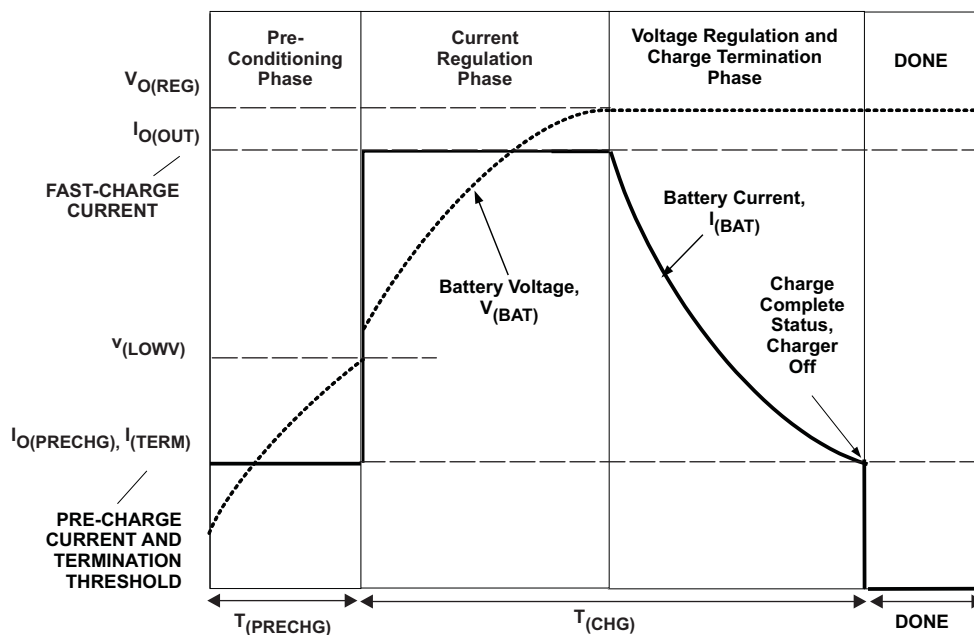
Figure 10. Charging Profile With T_{\text{J(REG)}}
