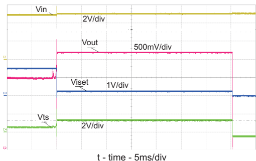
Figure 9. Battery Removal – GND Removed 1st, 42 \Omega Load
