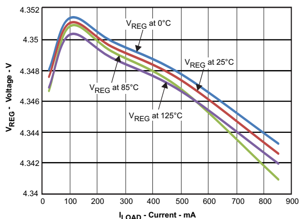
Figure 22. Load Regulation
