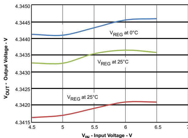
Figure 23. Line Regulation
