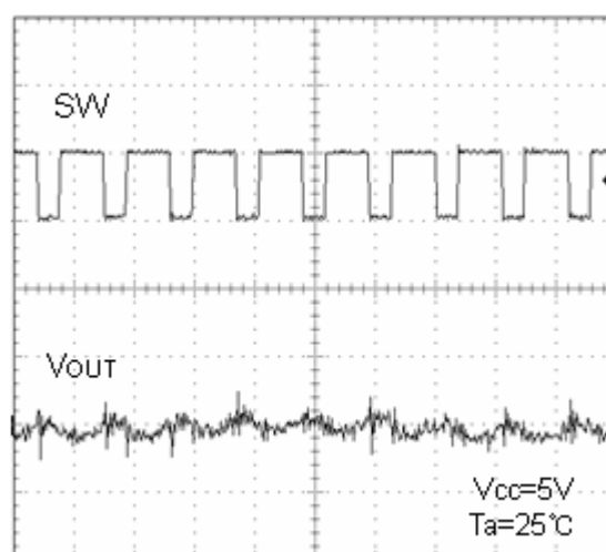
Fig.15 SW waveform
