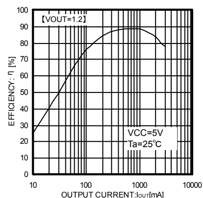
Fig.23 Efficiency
