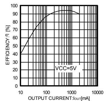
Fig.23 Efficiency
