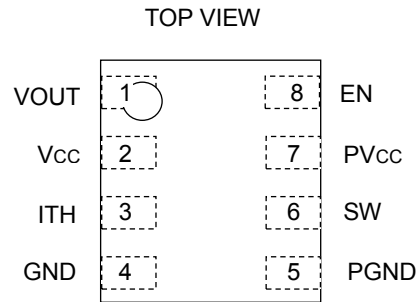
Fig.2 Pin Configuration
