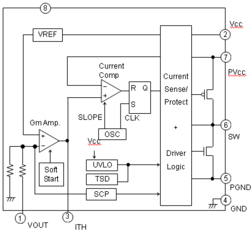
Fig.3 Block Diagram
