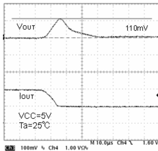
Fig.17 Transient response I_o=2A \rightarrow 1A(10\mu s)
