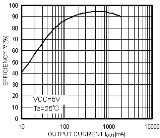
Fig.8 Efficiency
