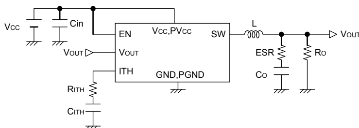
Fig.31 Typical application
