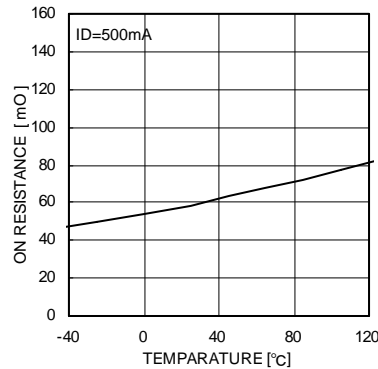
Fig.10. Nch FET ON resistance temperature property
