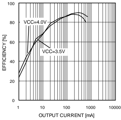
Fig.22 Power conversion efficiency 3
