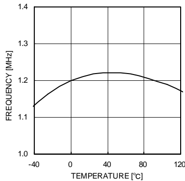
Fig.7. fosc temperature property
