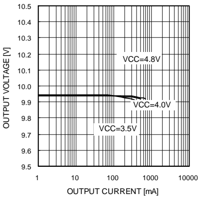
Fig.25 Load regulation 2
