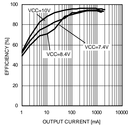
Fig.20 Power conversion efficiency 1
