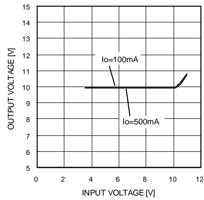
Fig.23 Line regulation
