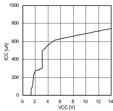
Fig.18. Circuit current power supply property
