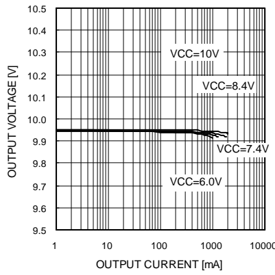
Fig.24 Load regulation 1
