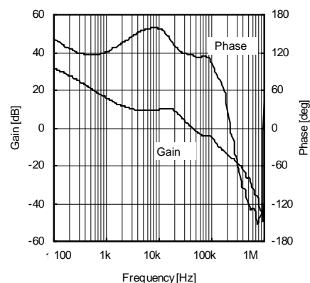
Fig.28 Frequency response property 3 (VCC = 8.4 V, Io = 200 mA)
