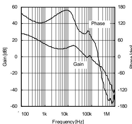
Fig.31 Frequency response property 6 (VCC = 8.4 V, Io = 500 mA)
