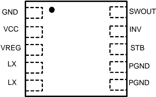
Fig.1 Pin layout
