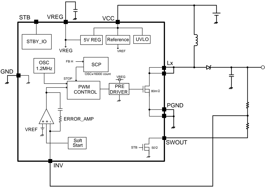
Fig.2 Block diagram
