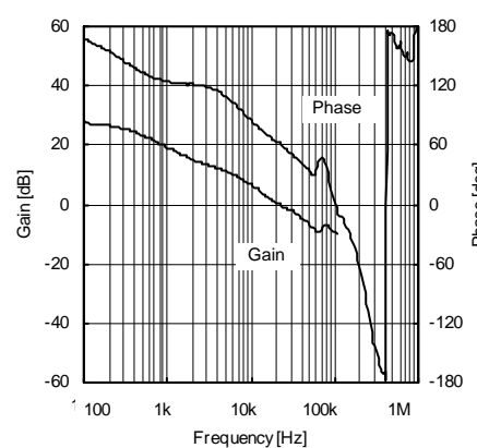
Fig.29 Frequency response property 4 (VCC = 3.0 V, Io = 500 mA)
