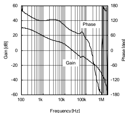
Fig.26 Frequency response property 1 (VCC = 3.0 V, Io = 200 mA)
