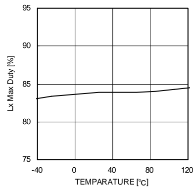
Fig.15. Lx Max duty temperature property
