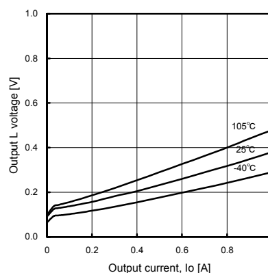
Fig.6 Output L voltage (Temperature characteristics)
