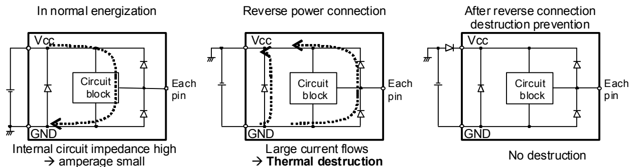
Fig.18 Flow of current when power is connected reversely
