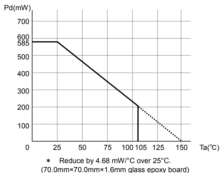
Fig.23 Thermal derating curve
