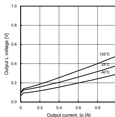
Fig.6 Output L voltage (Temperature characteristics)
