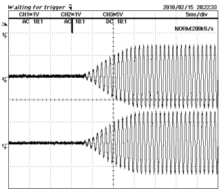
Fig.19 Advanced Switch 1
