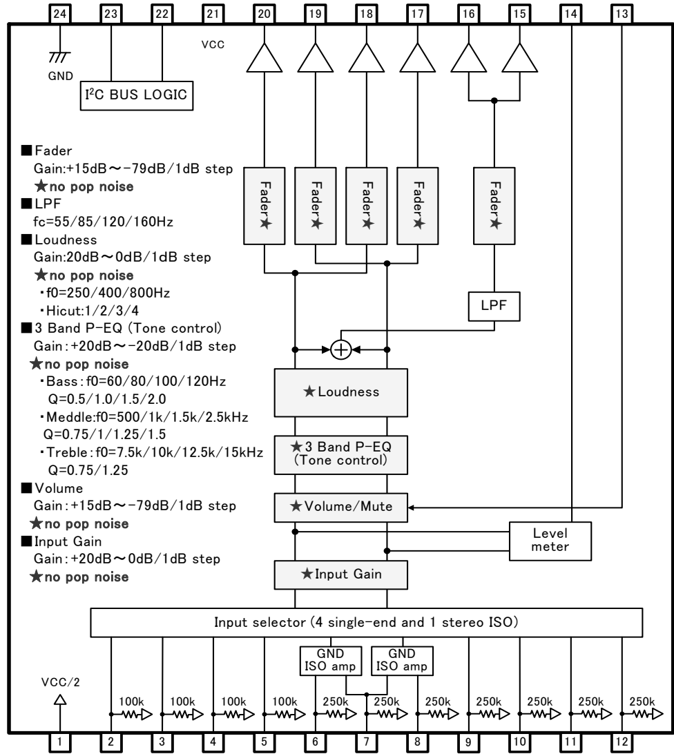
Fig.22 BD37524FS
