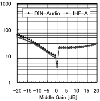
Fig.15 Middle Gain vs Noise
