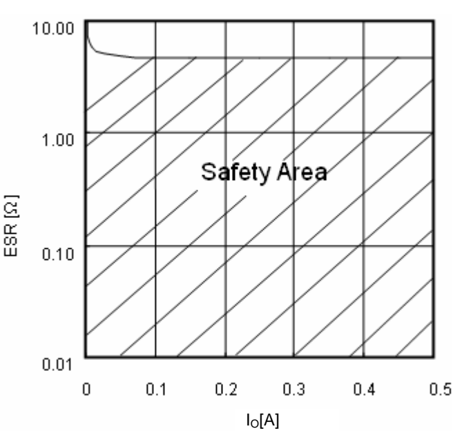
Fig.18 ESR condencer
