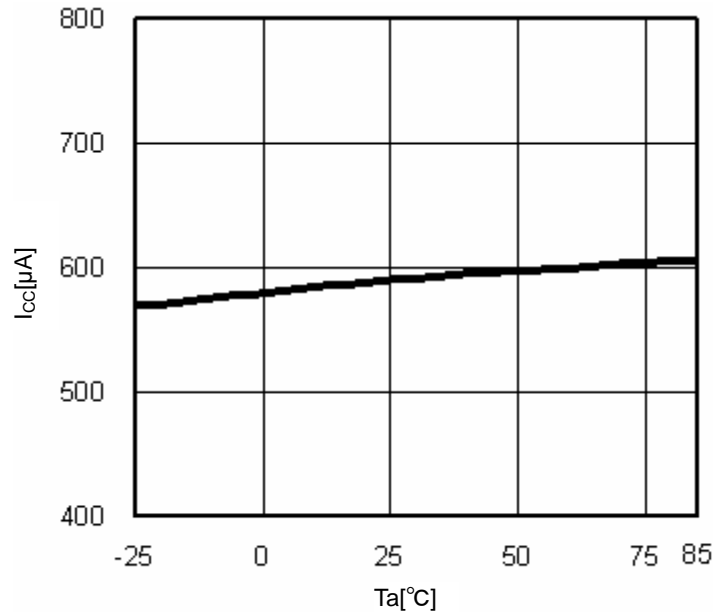
Fig.9 T<sub>a</sub>-I<sub>CC</sub>
