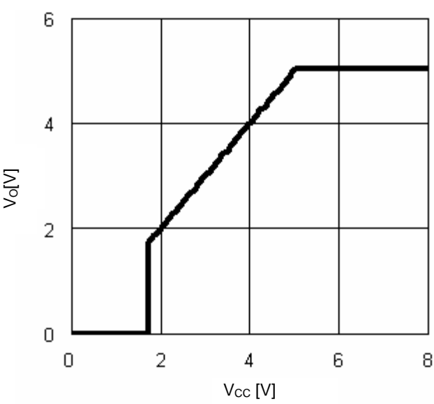
Fig.14 V_{CC}-V_O ( I_O=0mA )
