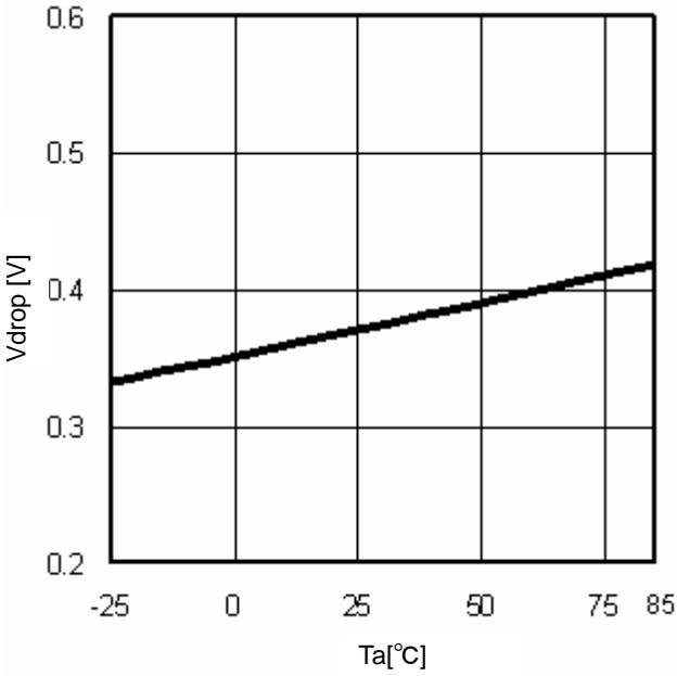
Fig.17 Minimum dropout Voltage1 ( V_{CC}=5V , I_O=-0.5A )
