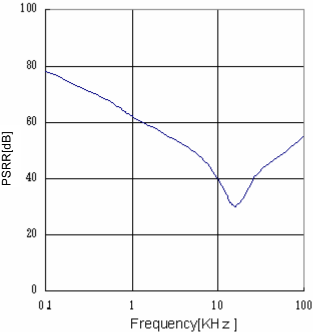
Fig.20 PSRR ( I_o=0mA )
