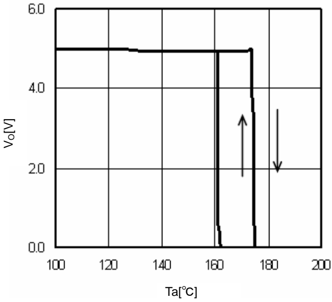
Fig.15 TSD ( I_O=0mA )
