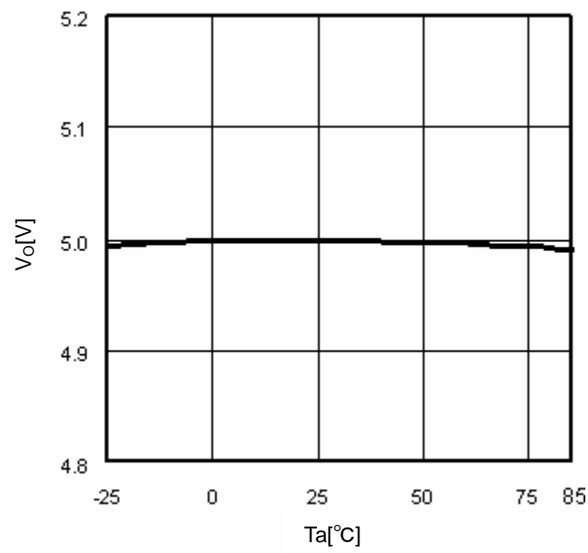
Fig.8 T<sub>a</sub>-V<sub>O</sub> (I<sub>o</sub>=0mA)
