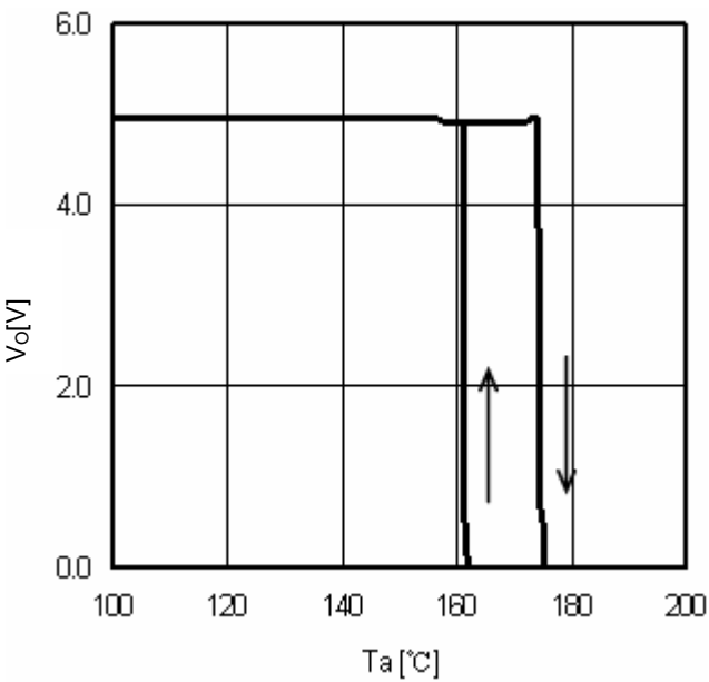
Fig.15 TSD ( I_o=0mA )
