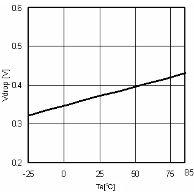
Fig.17 Minimum dropout Voltage ( V_{cc}=5V , I_o=-0.3A )
