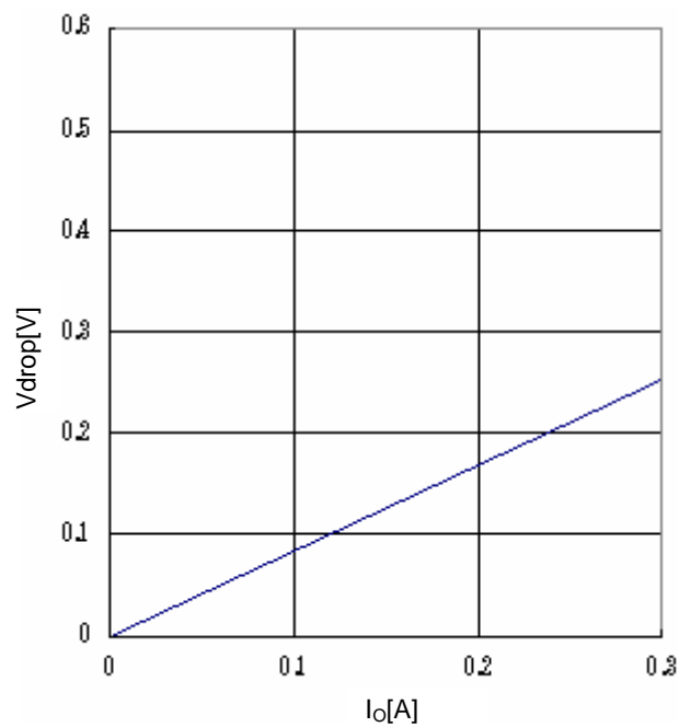
Fig.23 Minimum dropout Voltage 4 ( V_{CC}=8V , T_a=25^\circ C )
