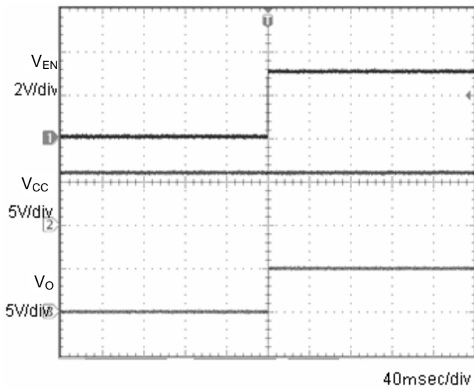
Fig.4 Input sequence 1 C_o=1\mu\text{F}
