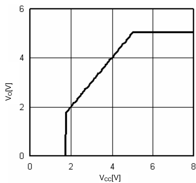
Fig.14 V_{cc}-V_o ( I_o=0mA )
