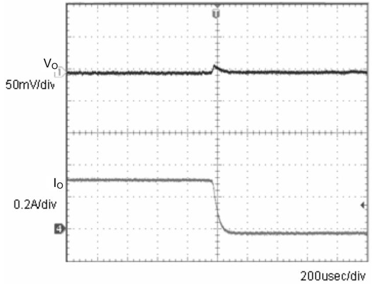
Fig.3 Transient Response (0.3→0A) C_o=1\mu\text{F}
