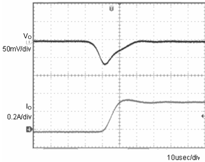
Fig.2 Transient Response (0→0.3A) C_o=1\mu\text{F}
