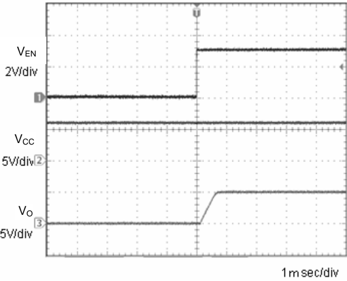
Fig.6 Input sequence 2 C_o=1\mu F
