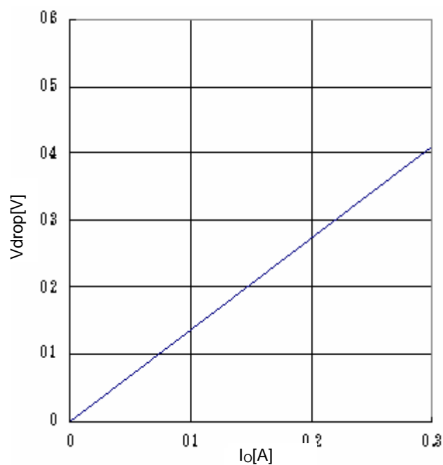
Fig.21 Minimum dropout Voltage 2 ( V_{CC}=4.5V , T_a=25^{\circ}C )
