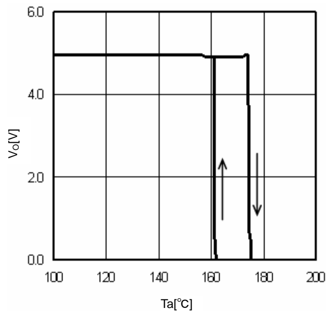
Fig.15 TSD ( I_o=0mA )
