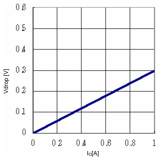
Fig.25 Minimum dropout Voltage 6 ( V_{CC}=12V , T_a=25^\circ C )
