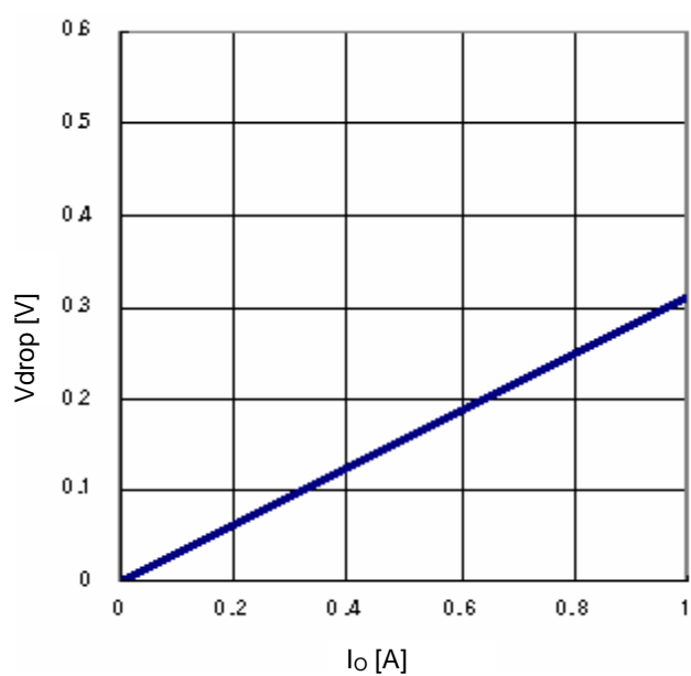
Fig.24 Minimum dropout Voltage 5 ( V_{CC}=10V , T_a=25^\circ C )
