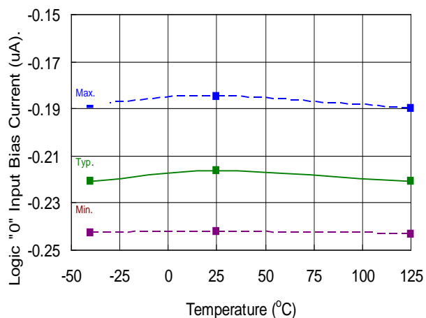
Figure 11. Logic "0" Input Bias vs Temperature
