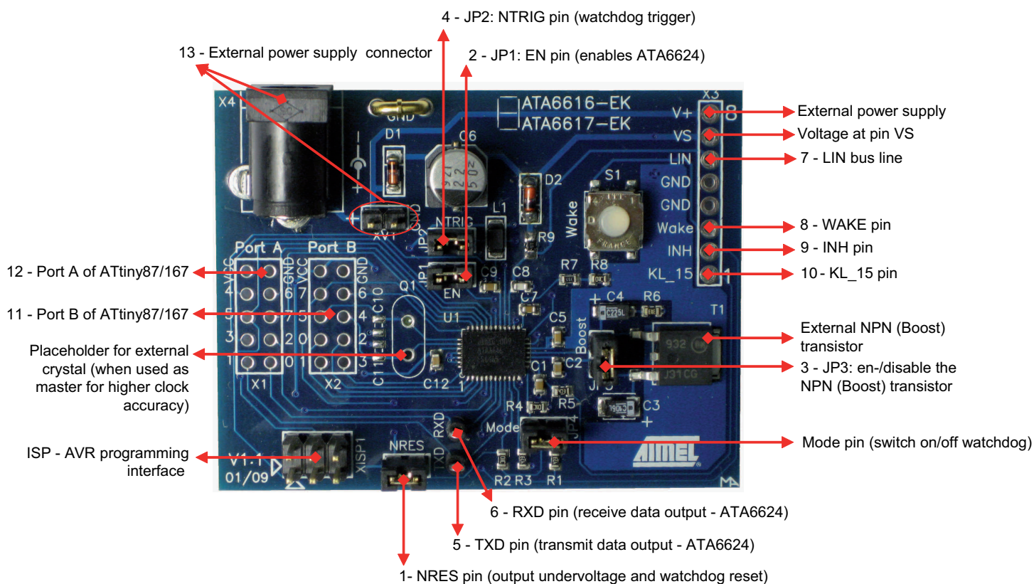
Figure 2-1. Atmel ATA6616/ATA6617 Development Board with Reference Points
