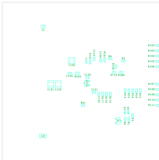
FIGURE 11. ASSEMBLY BOTTOM
