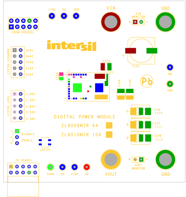
FIGURE 4. SILK SCREEN TOP
