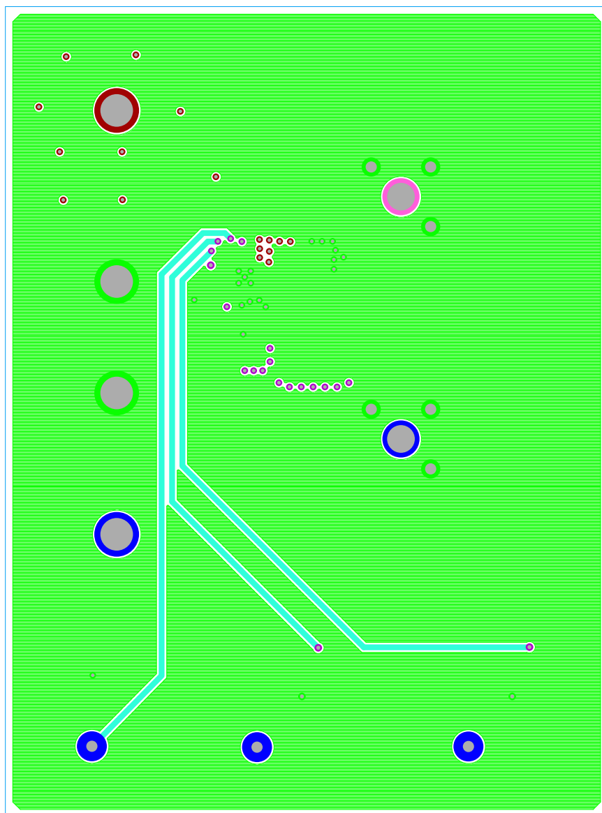
FIGURE 4. THIRD LAYER ETCH
