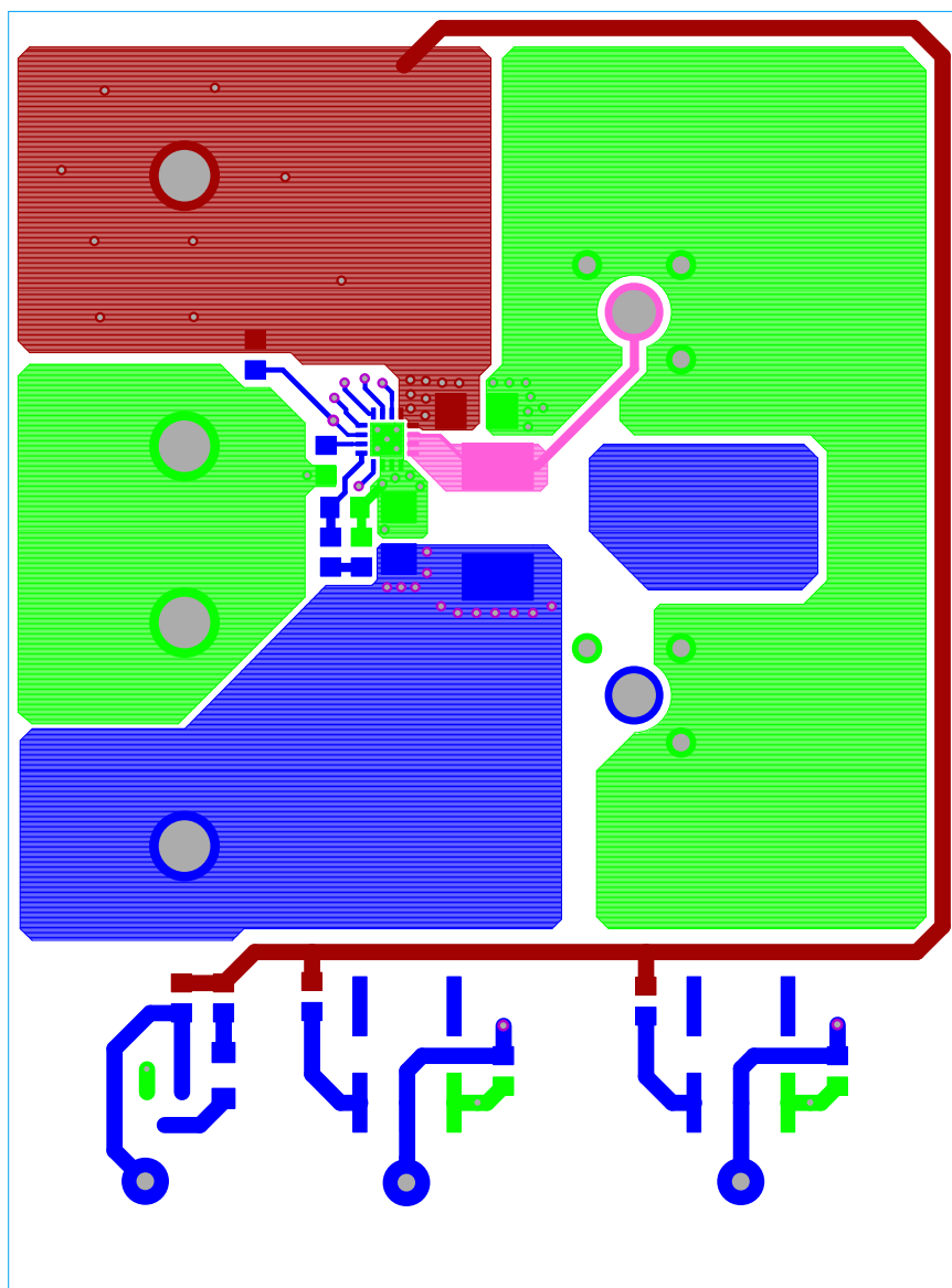
FIGURE 2. TOP LAYER ETCH
