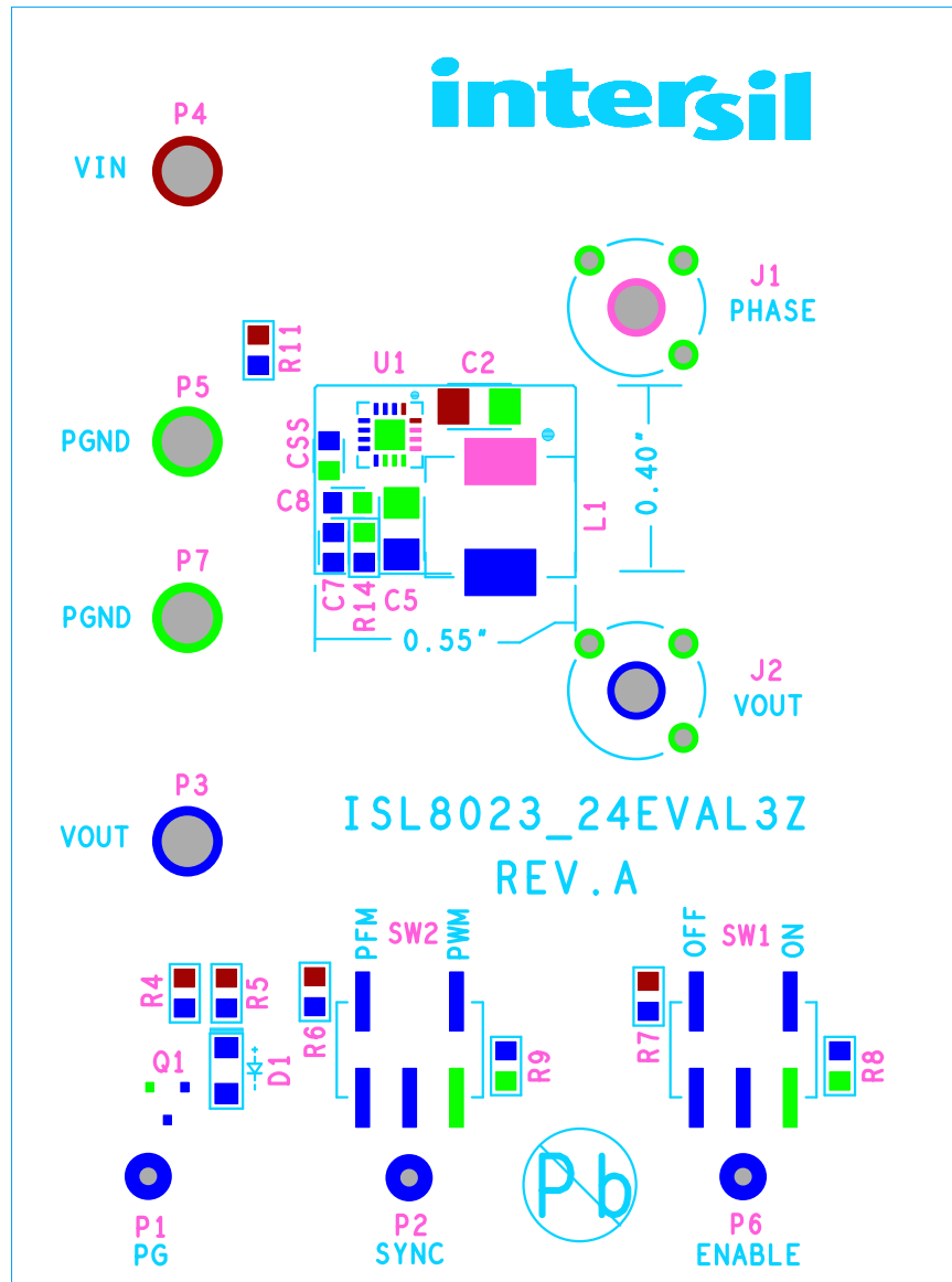
FIGURE 1. TOP LAYER COMPONENTS
