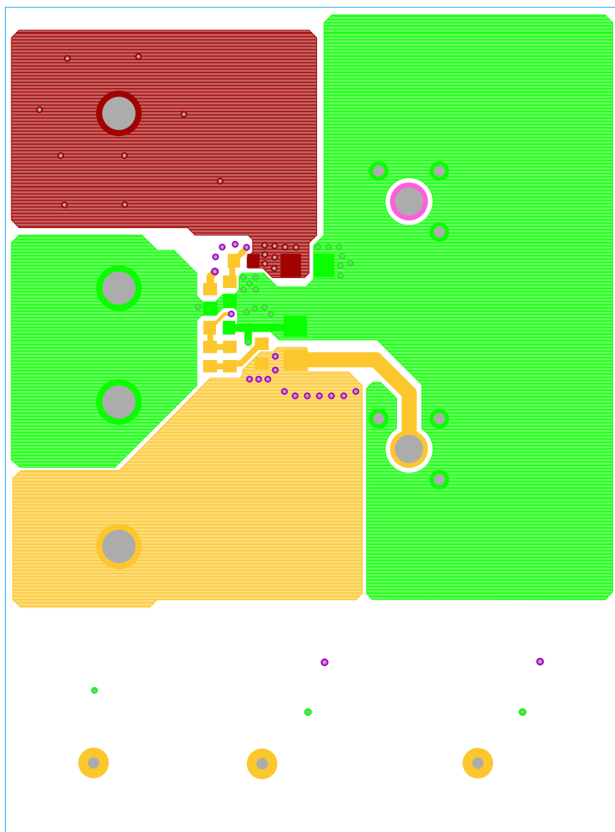
FIGURE 5. BOTTOM LAYER ETCH
