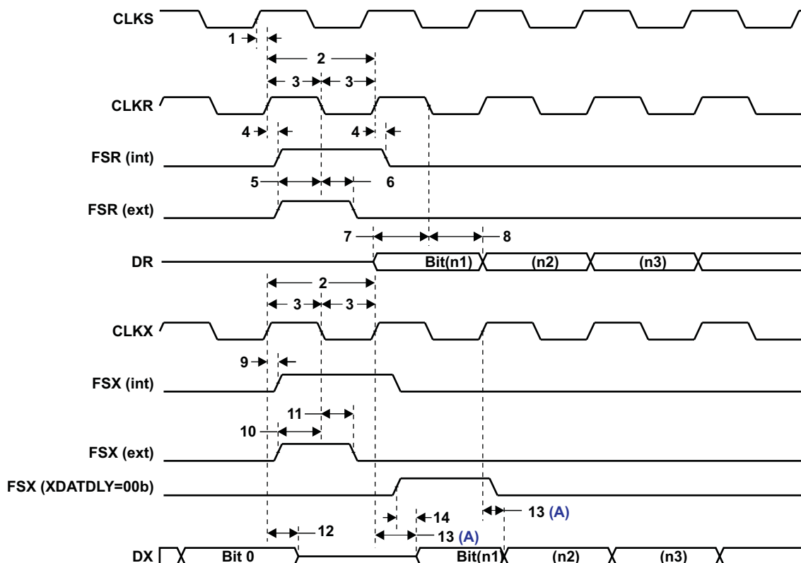
Figure 5-31. McBSP Timing
