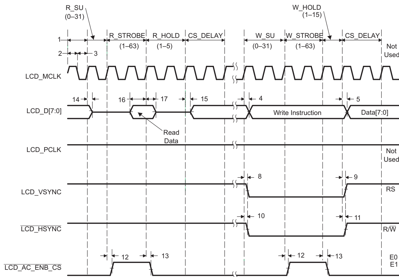
Figure 5-45. Character Display HD44780 Read
