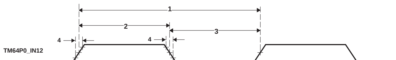
Figure 5-72. Timer Timing
