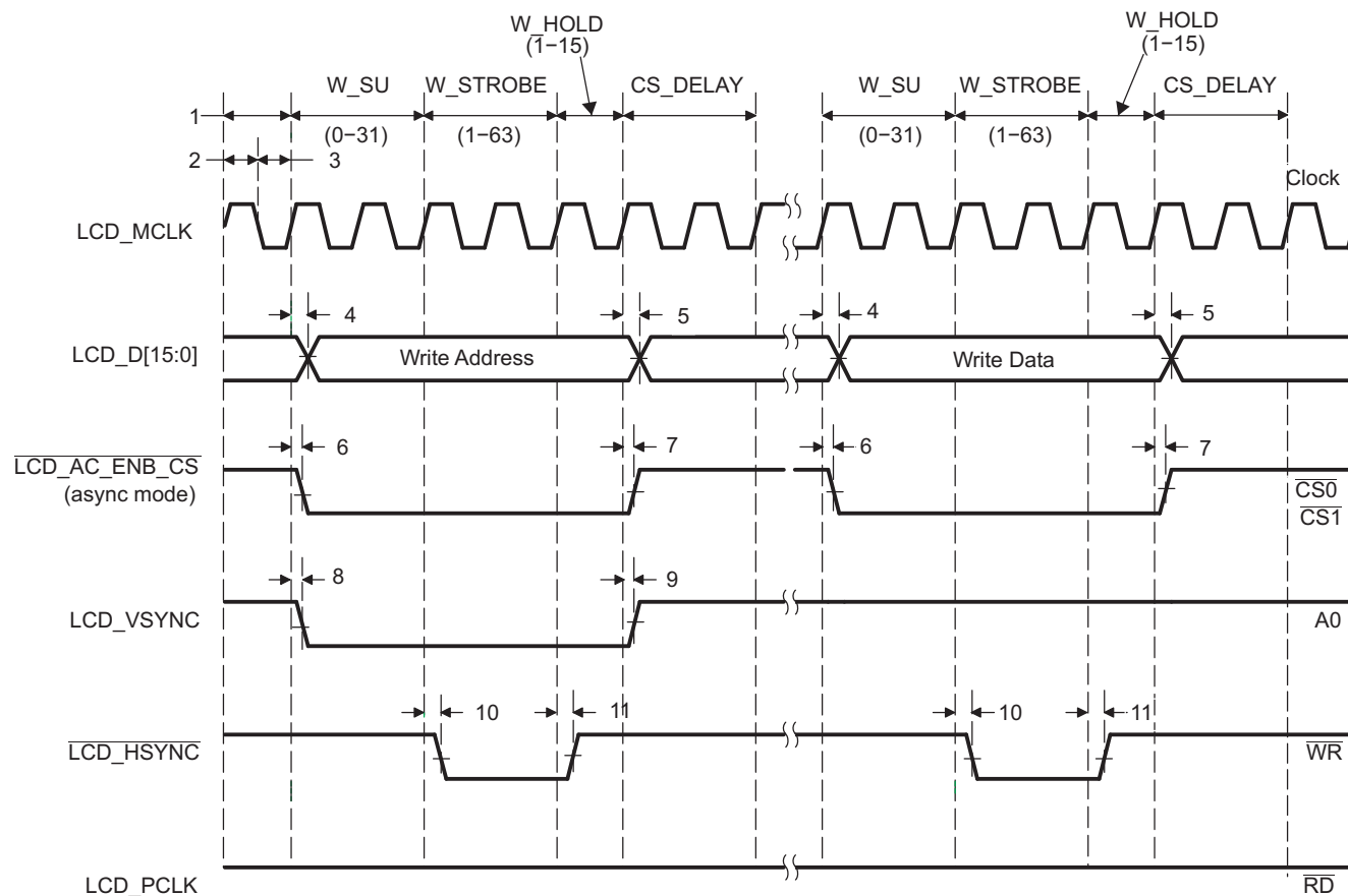
Figure 5-49. Micro-Interface Graphic Display 8080 Write
