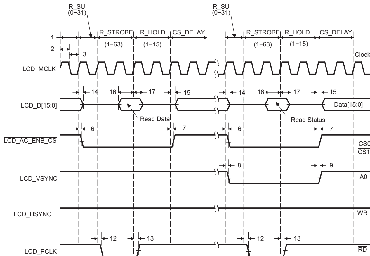
Figure 5-51. Micro-Interface Graphic Display 8080 Status
