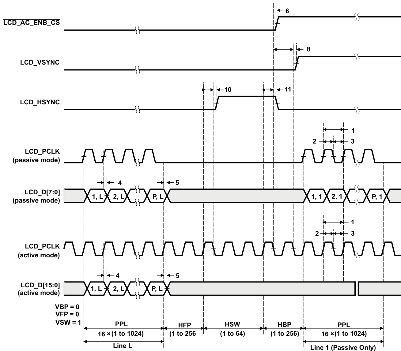
Figure 5-55. LCD Raster-Mode Control Signal Activation
