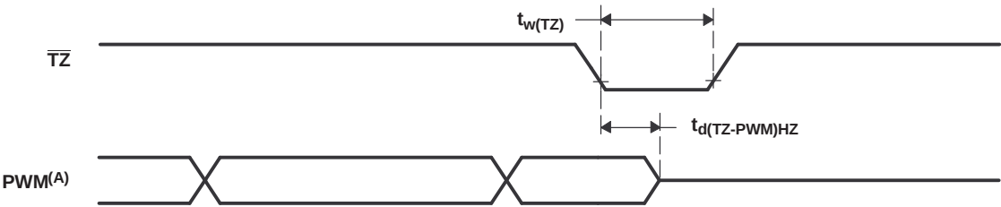
Figure 5-71. PWM Hi-Z Characteristics
