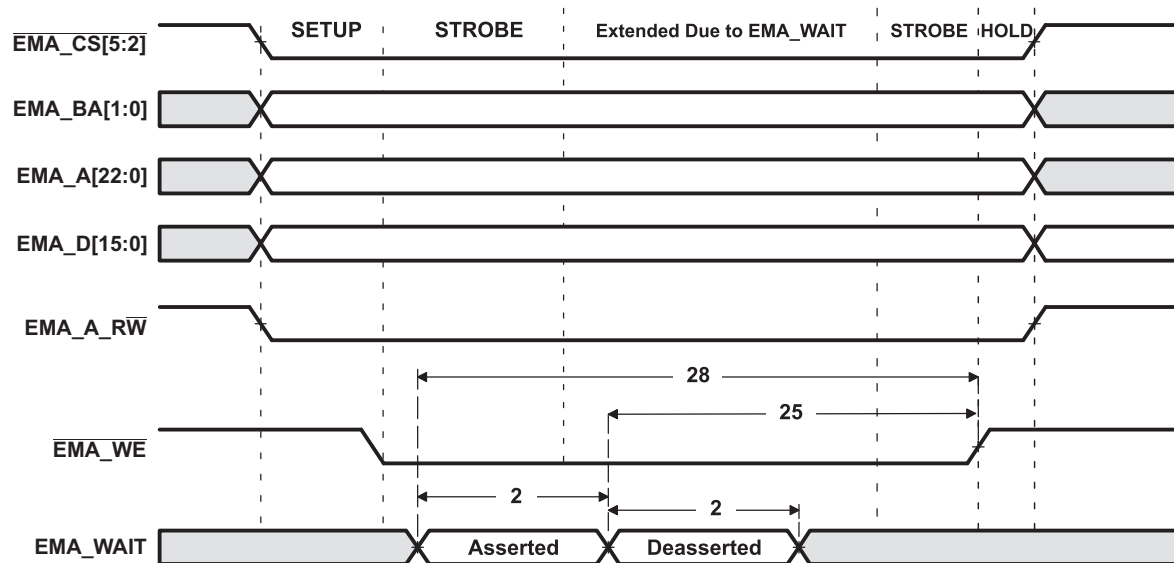
Figure 5-15. EMA_WAIT Write Timing Requirements
