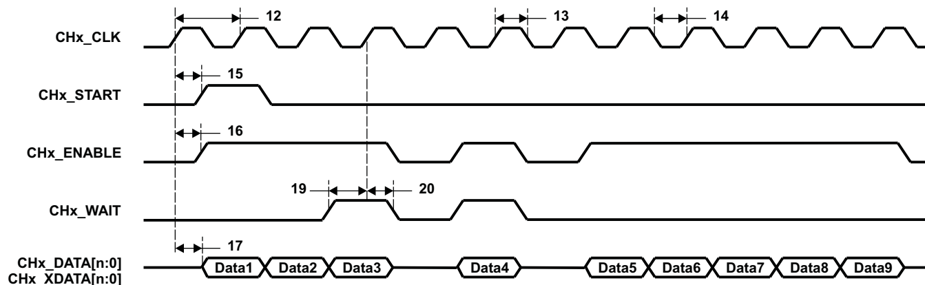
Figure 5-63. uPP Single Data Rate (SDR) Transmit Timing
