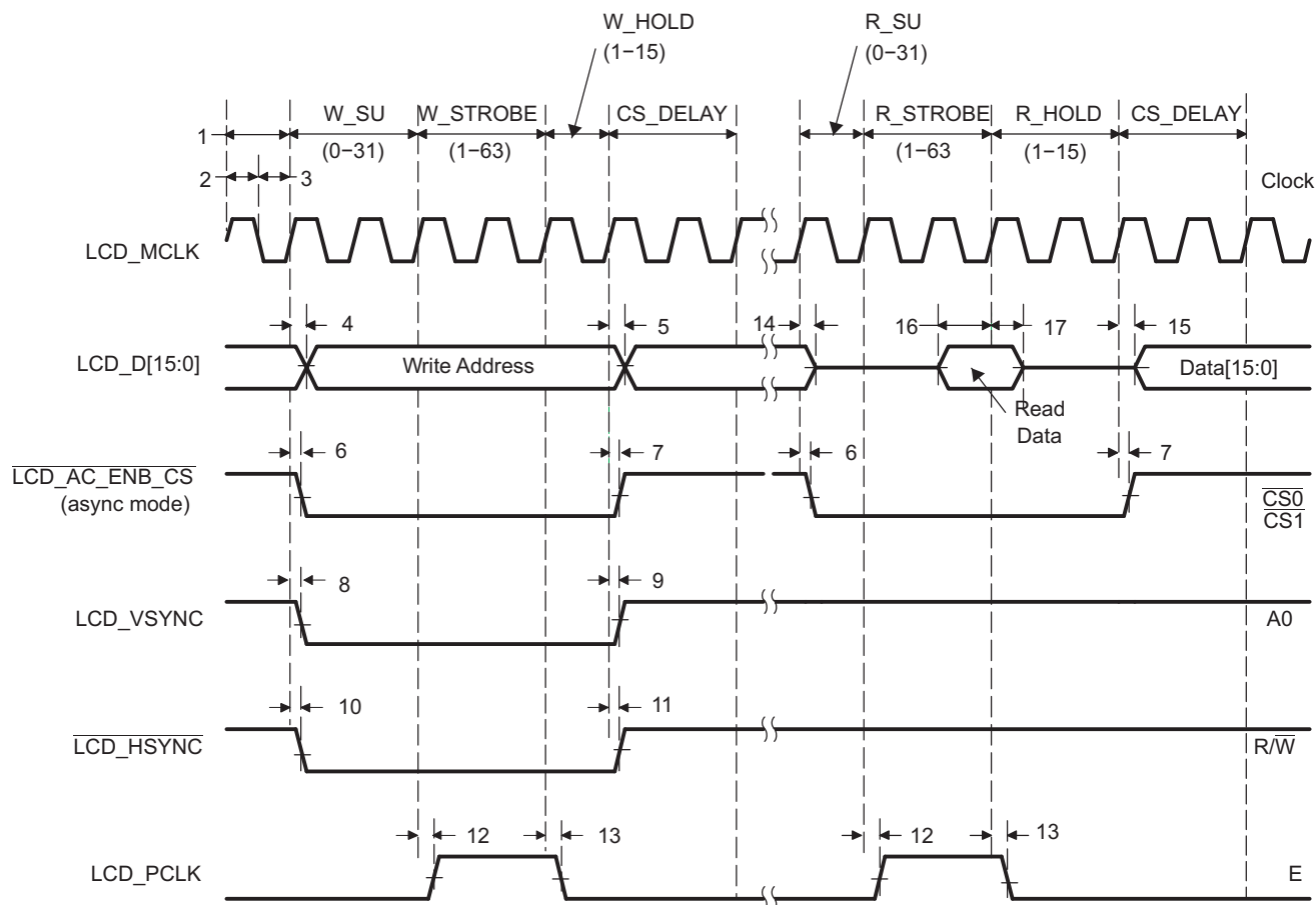
Figure 5-47. Micro-Interface Graphic Display 6800 Read
