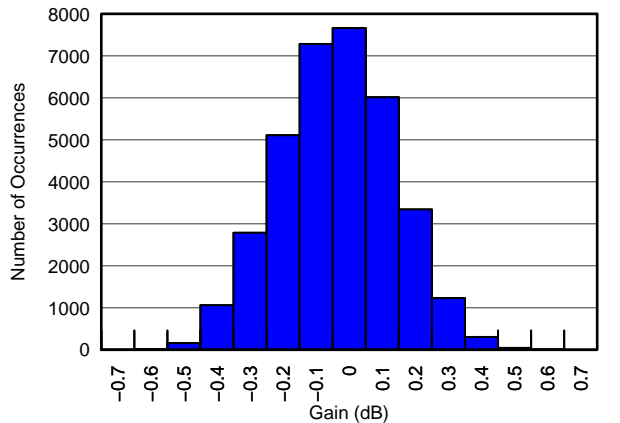
Figure 6. Gain Matching Histogram, VCNTL = 0.9V (34951 channels)
