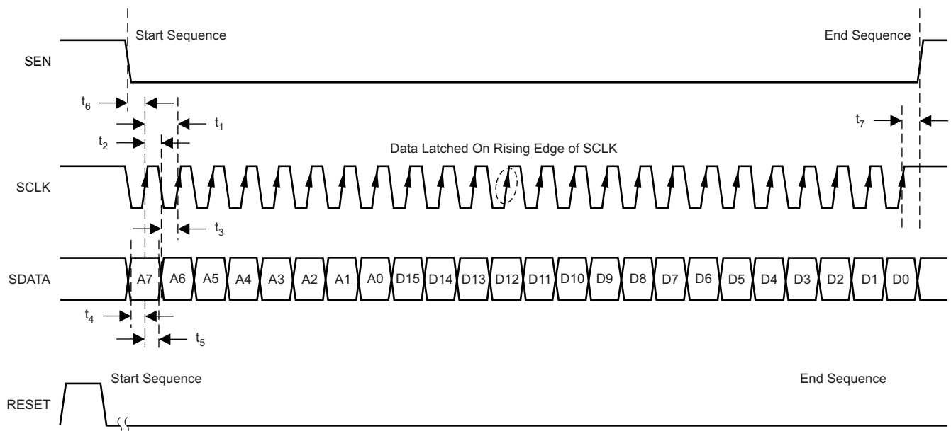
Figure 60. SPI Timing
