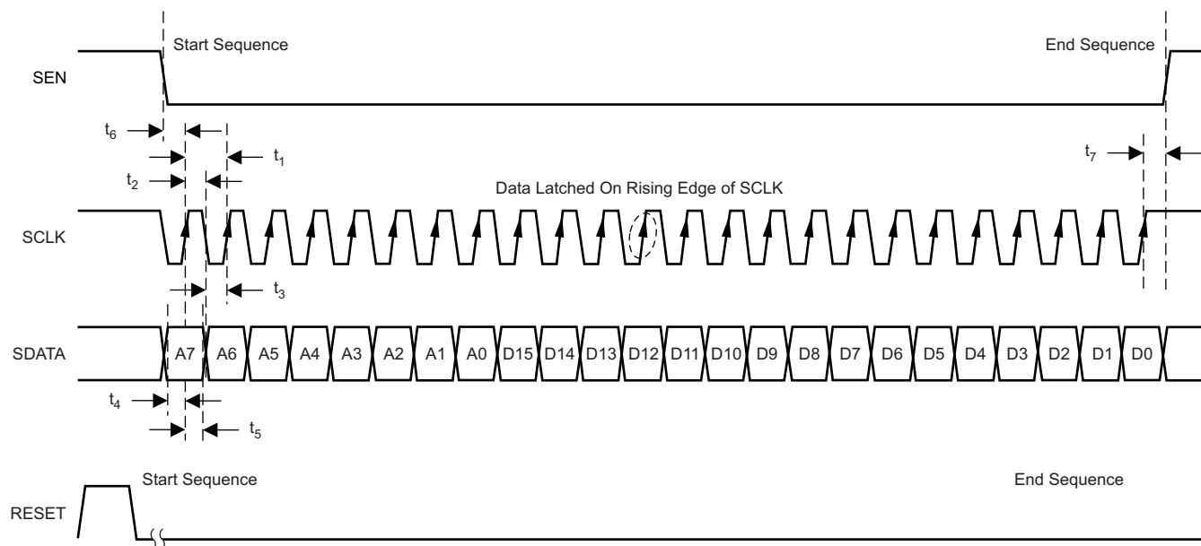
Figure 59. SPI Timing
