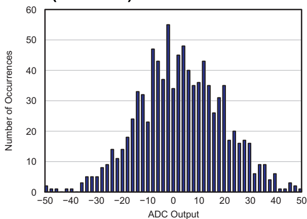
Figure 7. Output Offset Histogram, VCNTL = 0V (936 channels)
