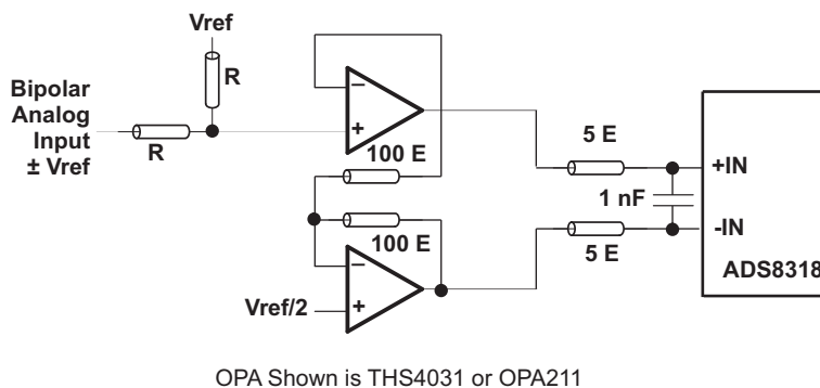
Figure 59. Bipolar Single-Ended Input Drive Configuration
