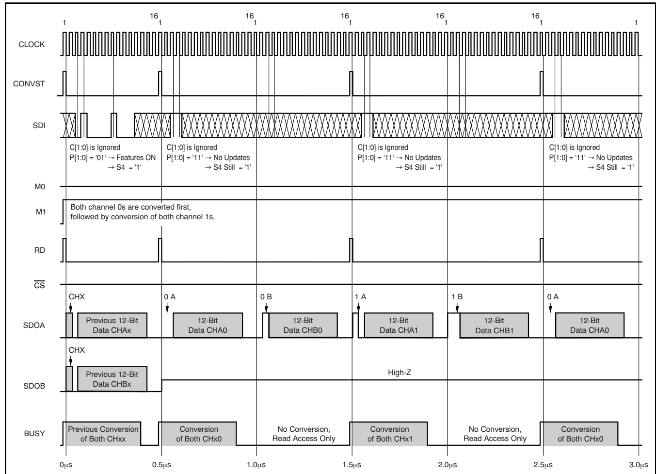
Figure 37. Special Mode IV Timing Diagram (M0 = 1; M1 = 1; S4 = 1)
