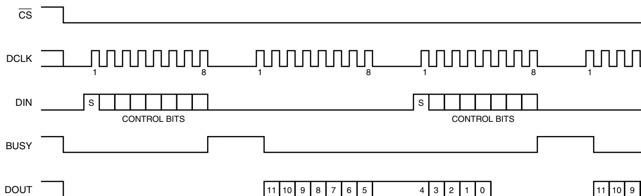
Figure 4. Conversion Timing
