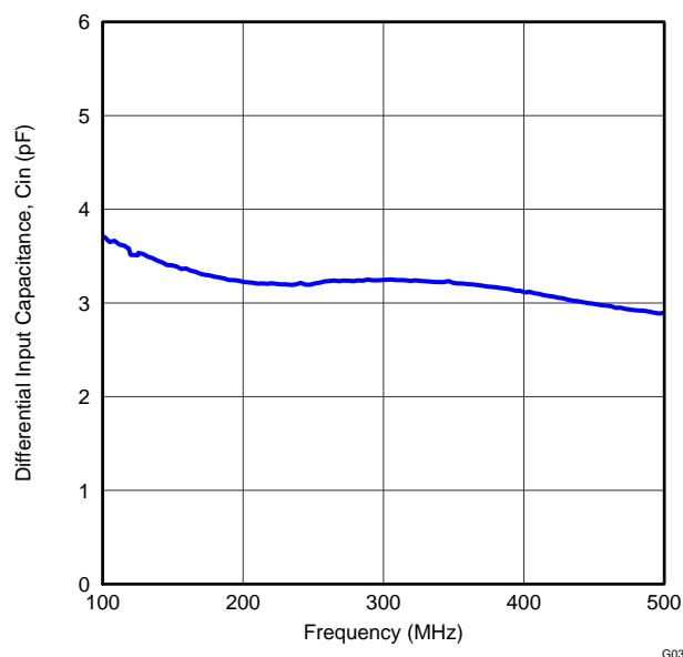
Figure 45. ADC Analog Input Capacitance ( C_{IN} ) vs Frequency
