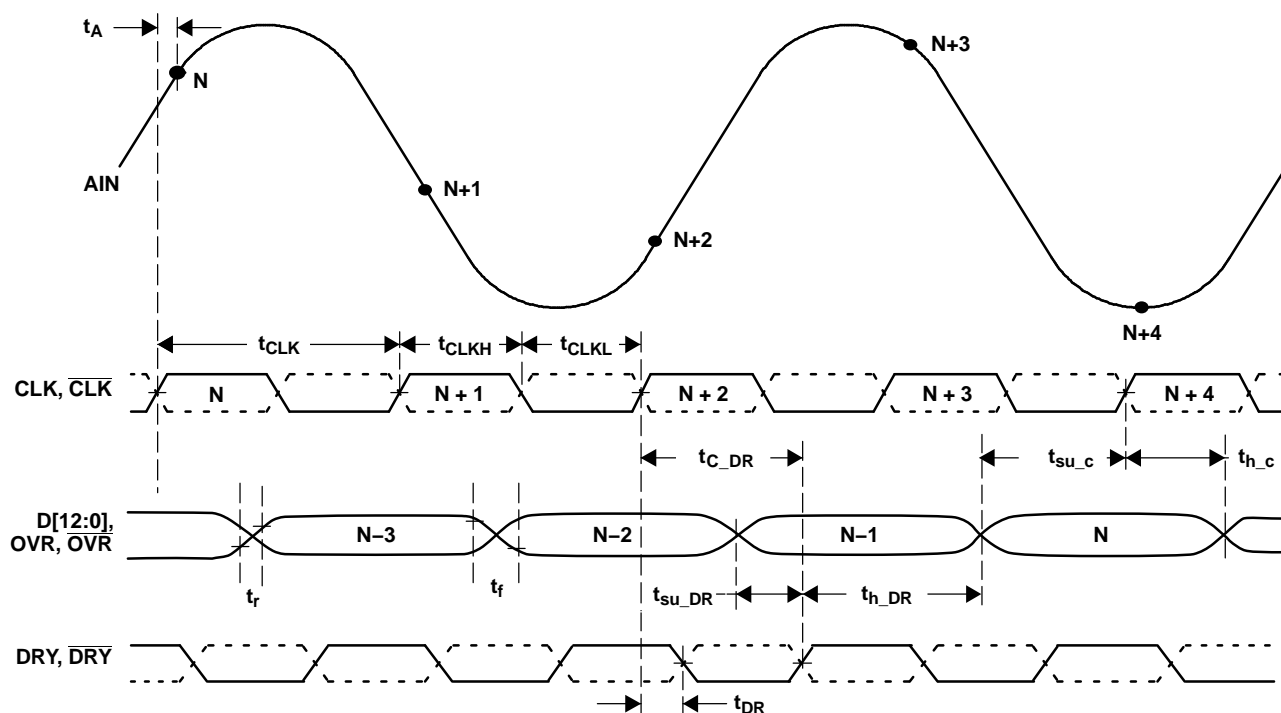
Figure 1. Timing Diagram
