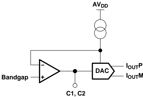
Figure 36. Decoupling Pin
