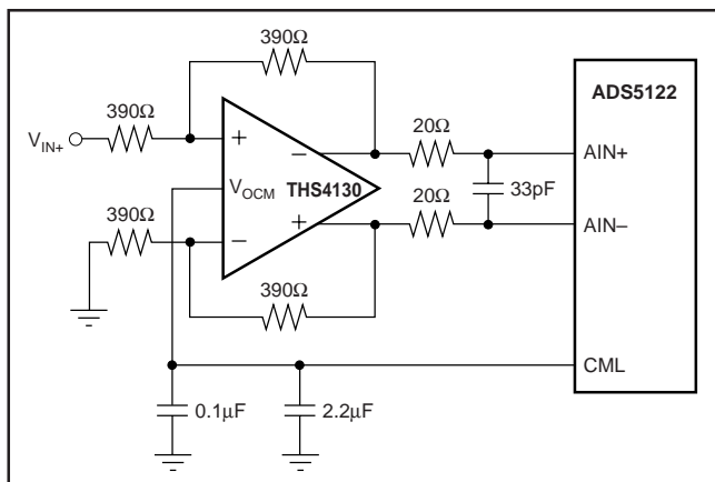
FIGURE 3. DC-Coupled Interface Using Differential I/O Amplifier TMS4130.
