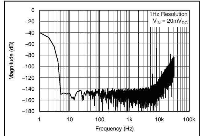
Figure 37. Modulator Output Spectrum
