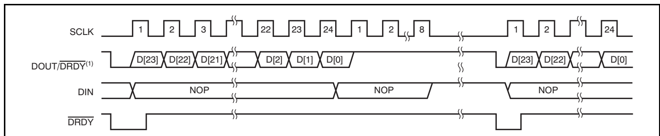
Figure 71. DOUT/DRDY Forced High After Retrieving the Conversion Result
