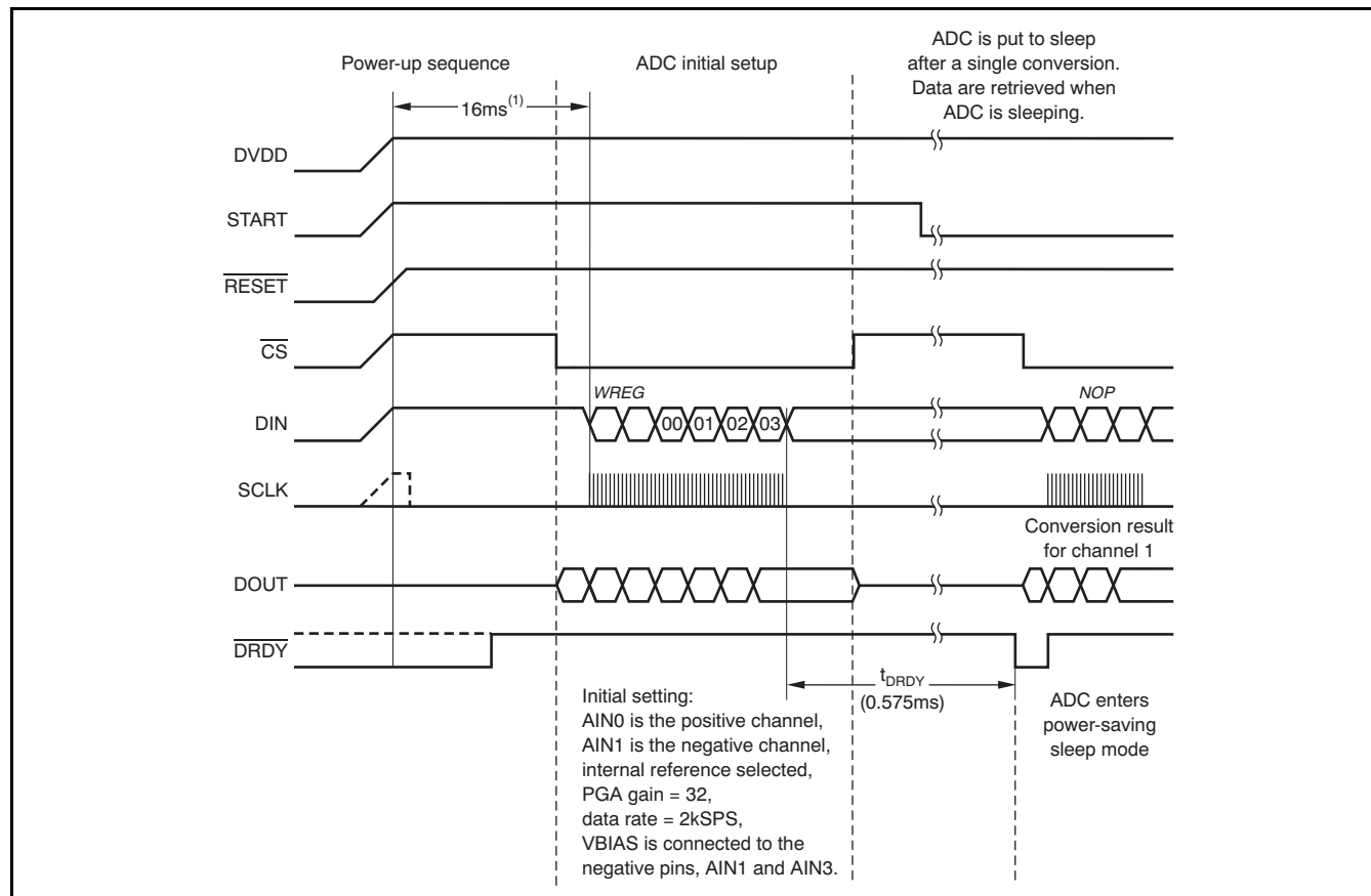
Figure 84. SPI Communication Sequence for Entering Sleep Mode After a Conversion
