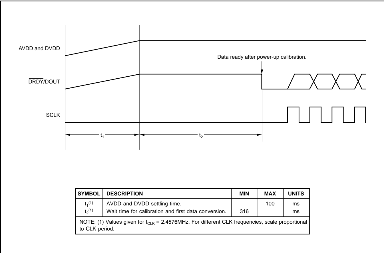
FIGURE 11. Power-Up Timing.
