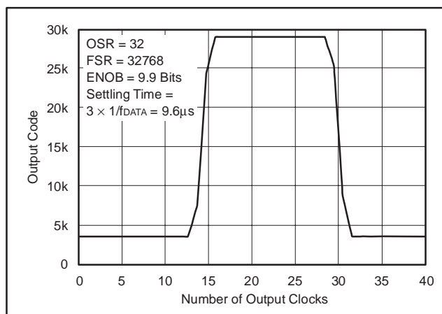
Figure 11. Pulse Response of Sinc 3 Filter ( f_{MOD} = 10\text{MHz} )
