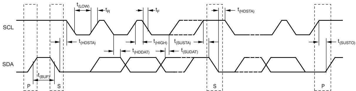
Figure 6. I²C Timing Diagram
